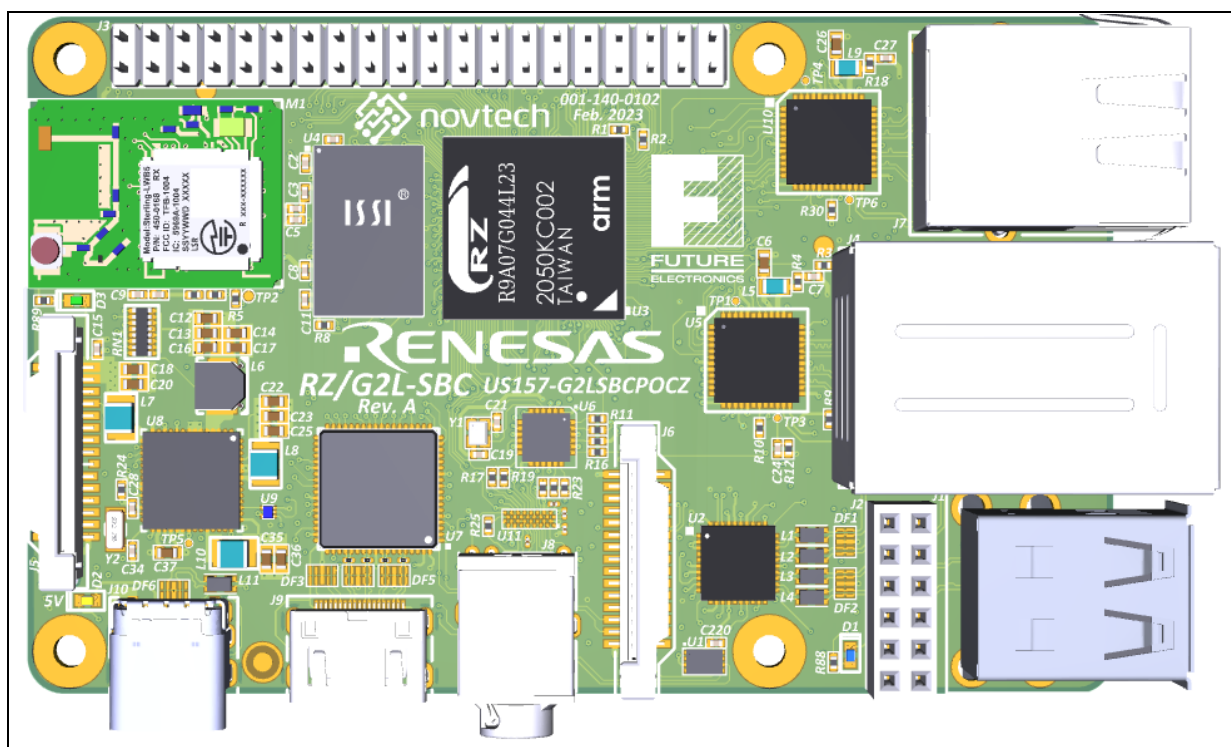
Figure 76. Top-side view of the RZ/G2L-SBC
