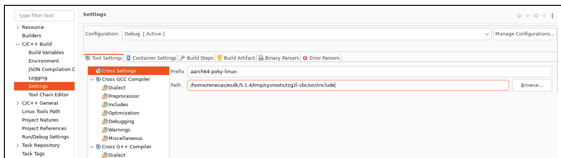
Figure 61. Configuring cross compiler settings in Eclipse tool settings
