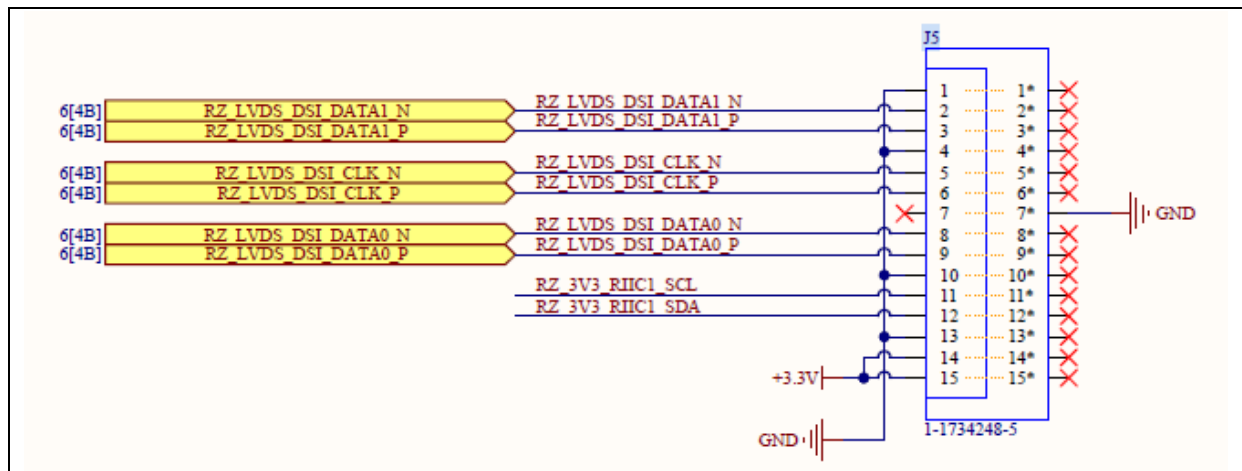
Figure 91. DSI Schematic
