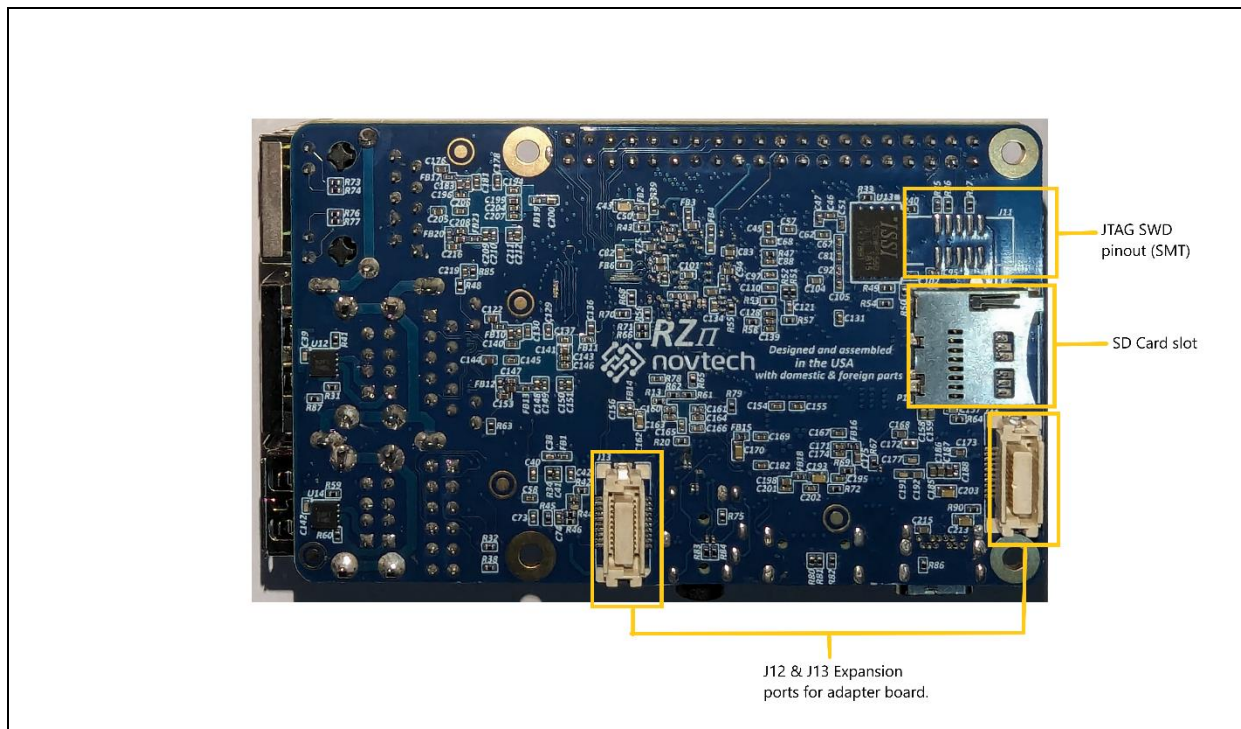
Figure 56: RZ/G2L-SBC Bottom view connectors.
