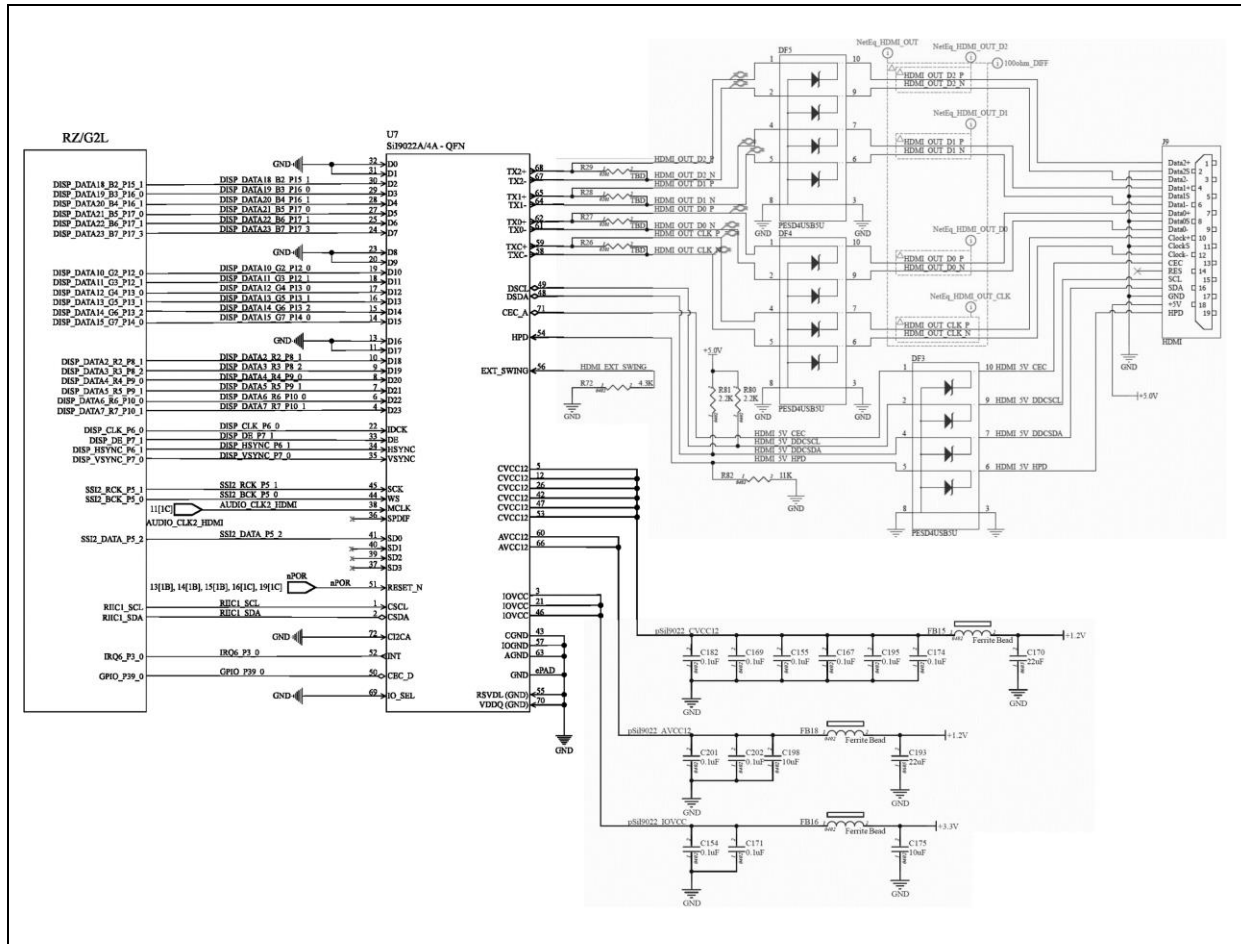
Figure 70: HDMI Bridge and mini HDMI port interfacing.
