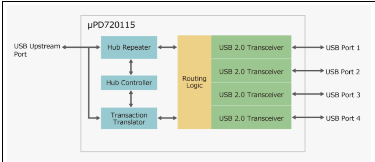
Figure 65: UPD720115 block diagram.
