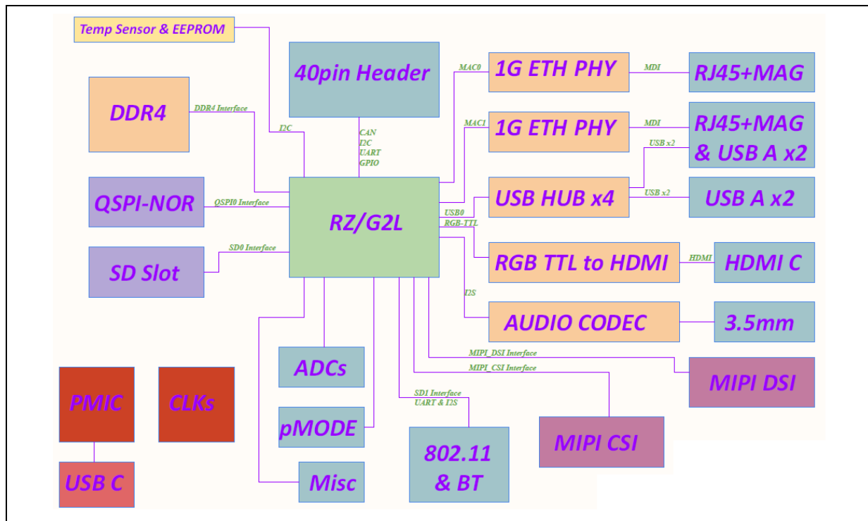
Figure 51: RZ/G2L SBC System Overview
