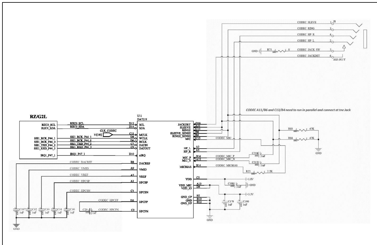
Figure 69: Audio CODEC Interface Block Diagram
