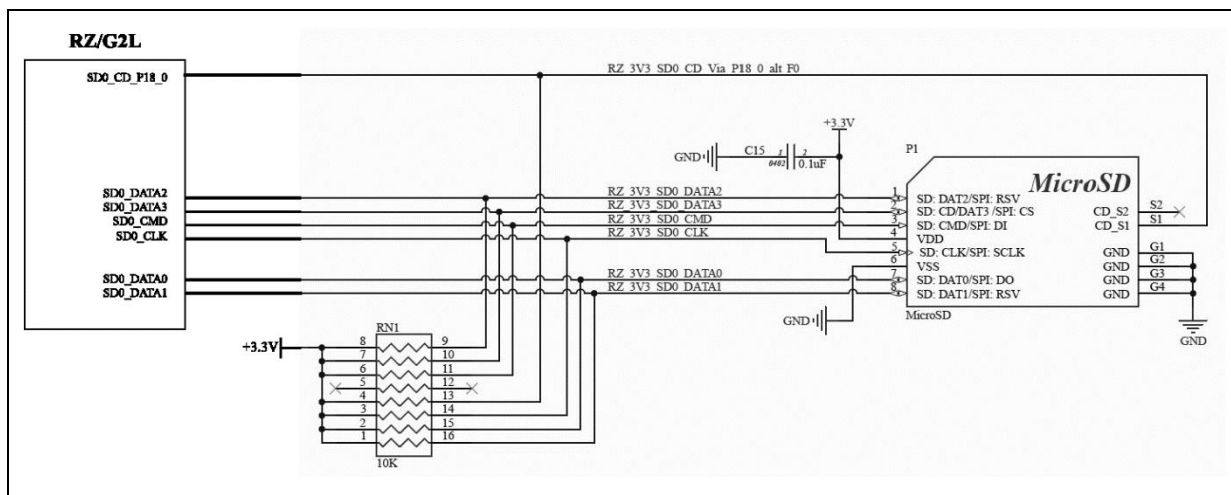
Figure 74: uSD-Card interface block diagram.
