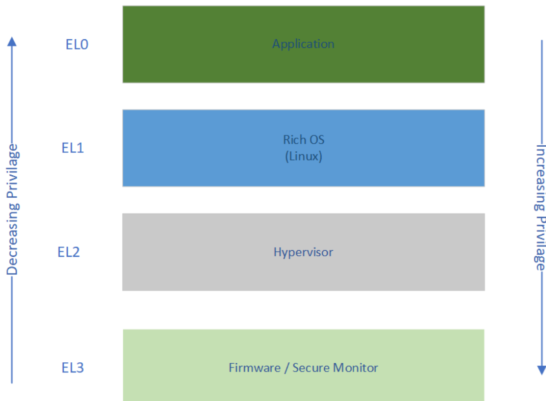
Figure 6: Arm Exception levels
