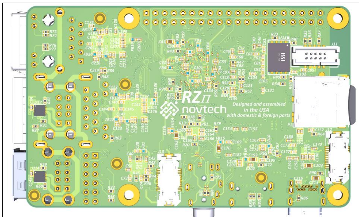
Figure 54: Bottom side of the RZ/G2L-SBC
