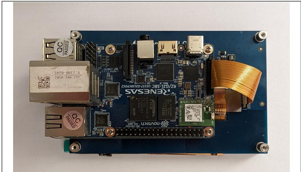
Figure 14: RZ/G2L-SBC mounted to the Waveshare DSI panel and interfaced.
