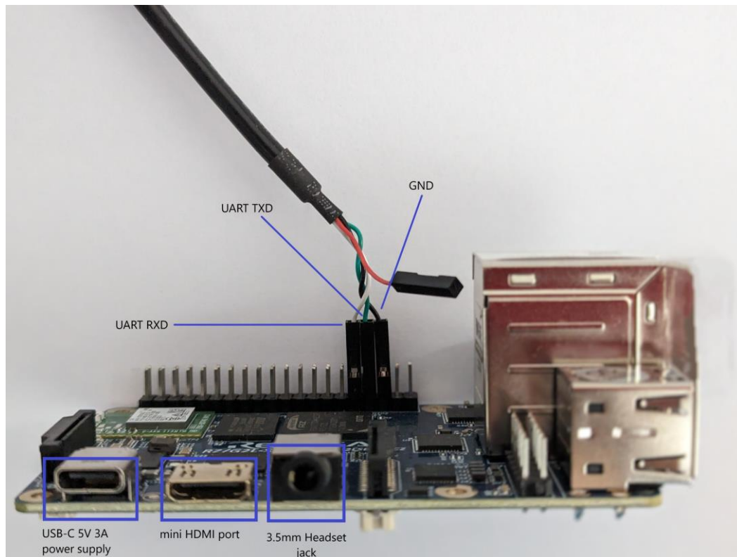
Figure 3: Essential minimum interfaces needed
