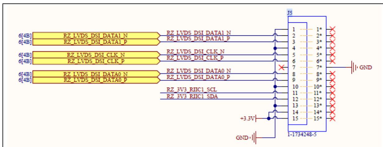
Figure 68: DSI Schematic
