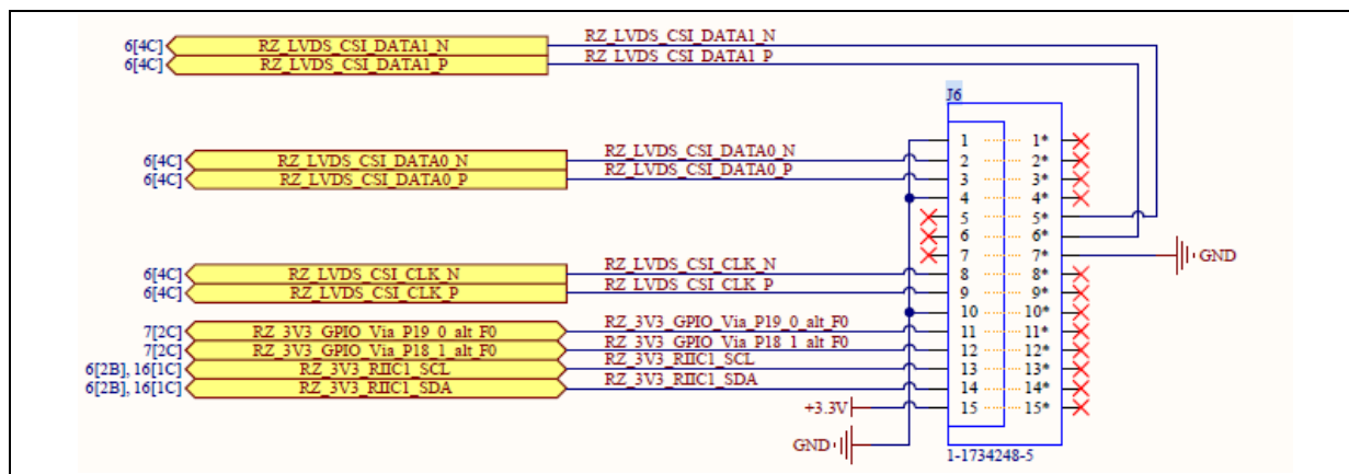
Figure 67: CSI Interface Schematic
