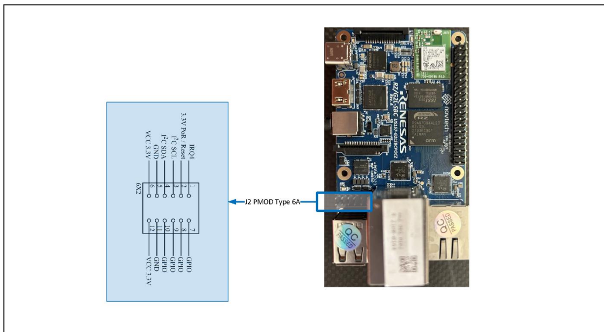
Figure 73: PMOD Type 6A 2x6 0.1mm pin out with orientation details.
