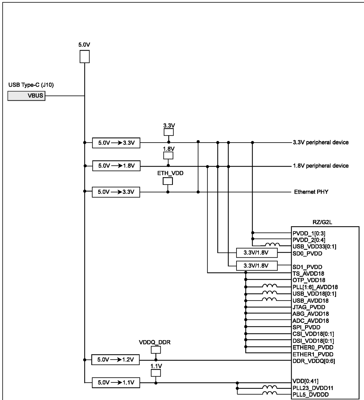
Figure 58: Power supply rails.
