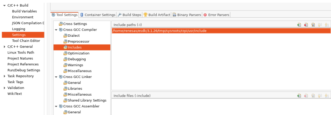
Figure 38: Configuring includes path in Eclipse tool settings
