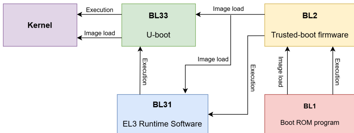
Figure 7: Trusted boot flow
