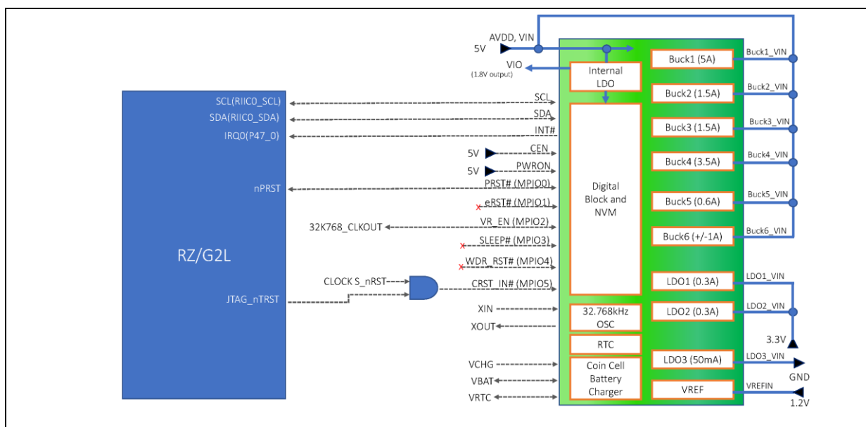
Figure 60: Block diagram of PMIC interface to RZ/G2L
