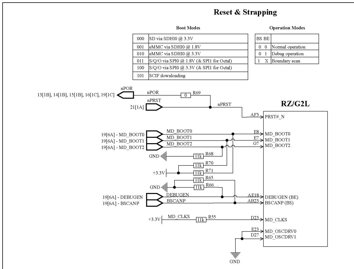
Figure 61: Reset Control Logic
