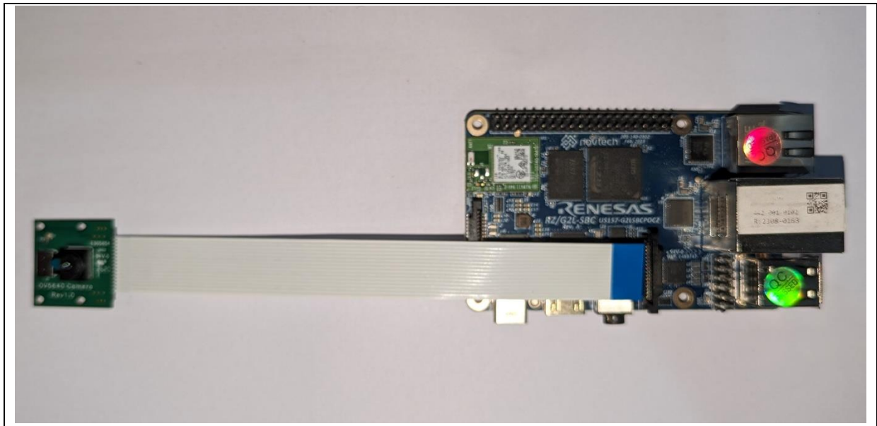
Figure 18: Orientation of the camera module. Blue stripe upward.
