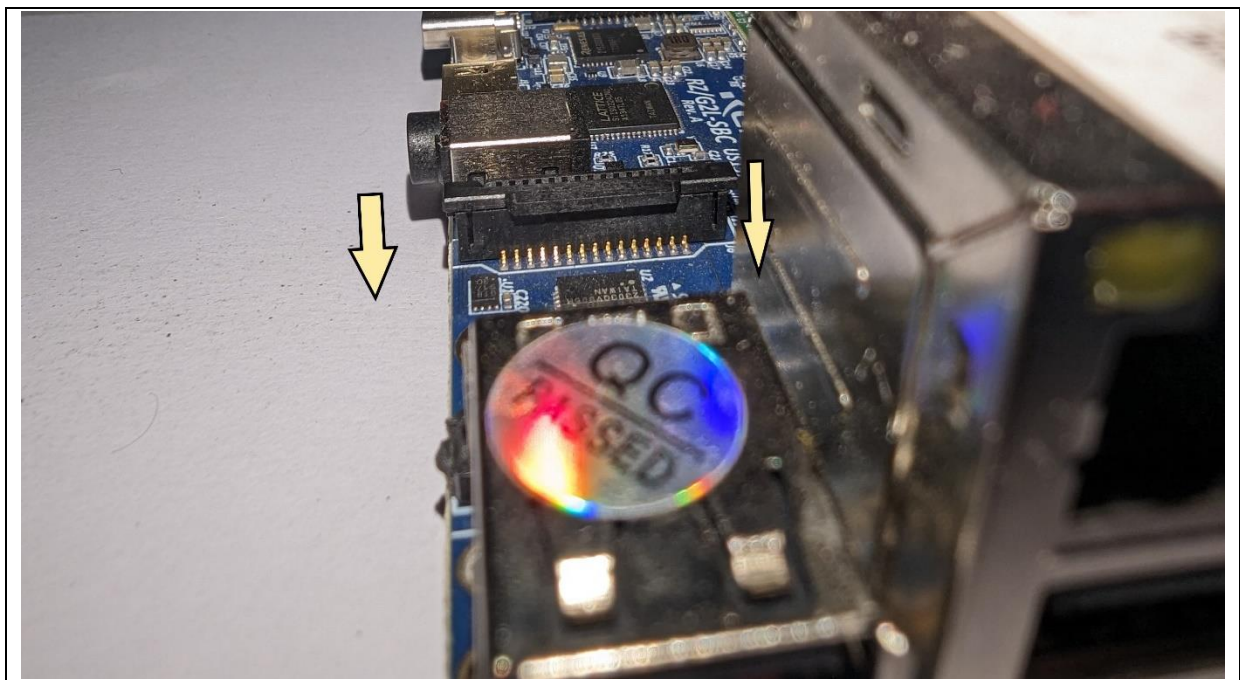
Figure 21: Push down the notch to lock it when you have inserted the flat cable
