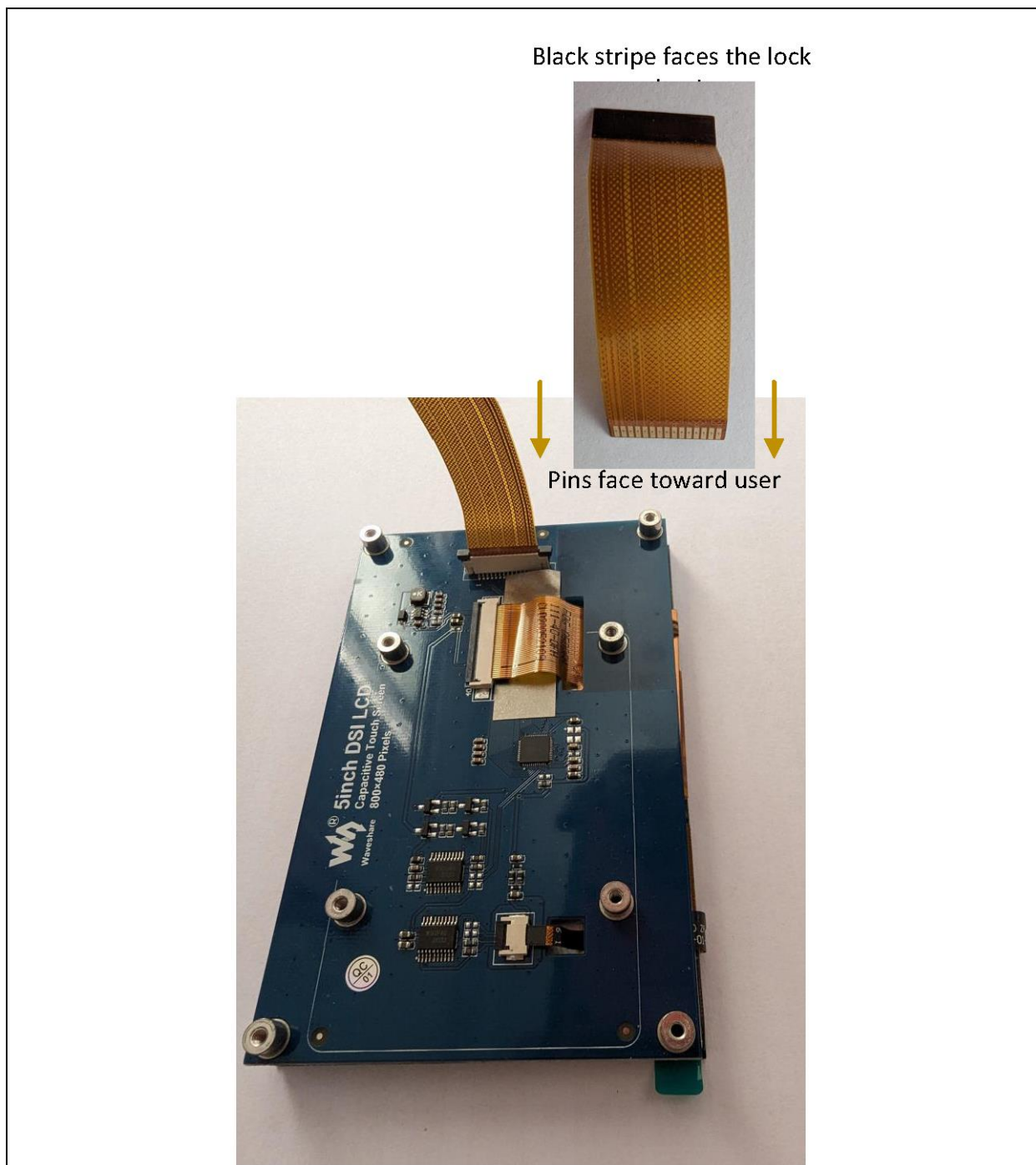
Figure 13: Waveshare DSI touch display DSI port interfacing cable orientation.
