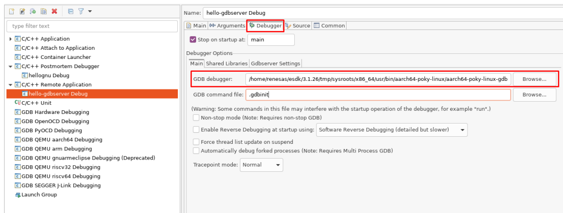
Figure 44: Configuring GDB debugger in Eclipse debug configurations
