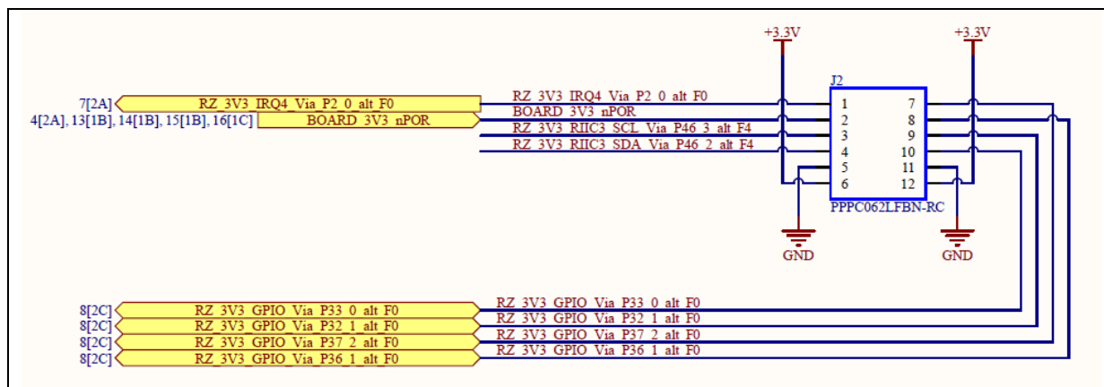
Figure 72: Schematic of PMOD Type 6 A pin header J2.
