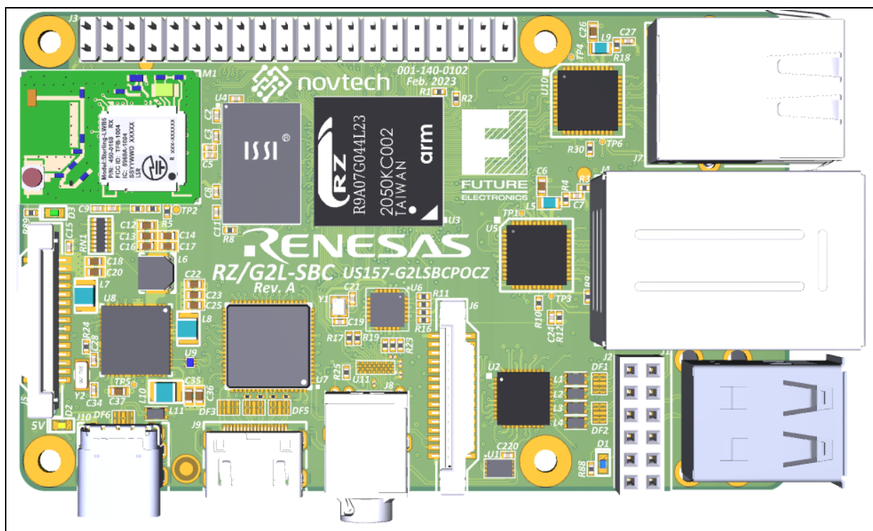
Figure 53: Top side view of the RZ/G2L-SBC
