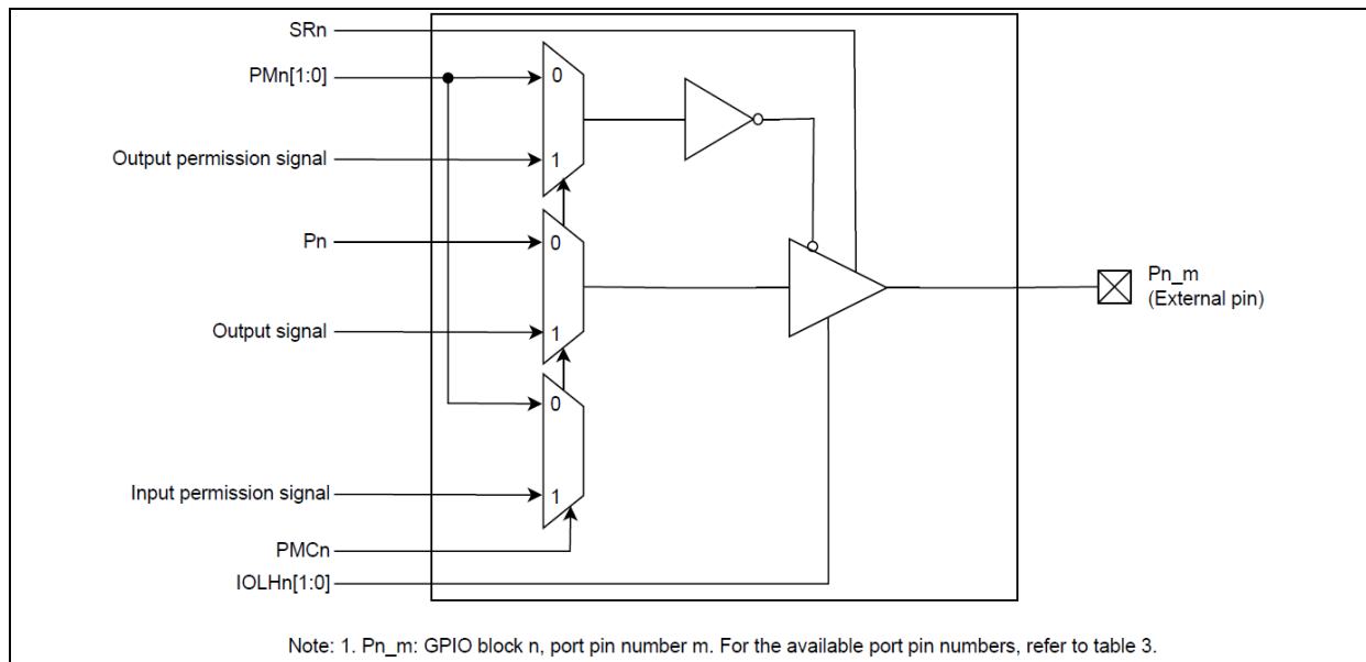
Figure 80: Multiplexed peripheral functions configuration diagram for GPIO pins
