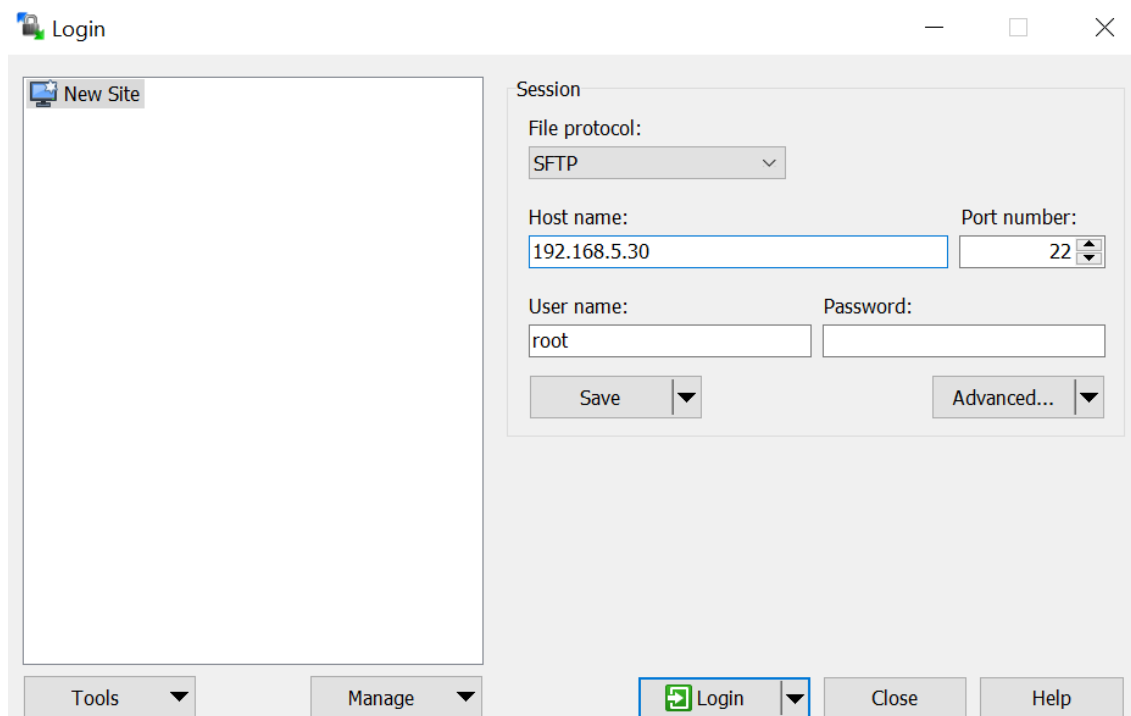
Figure 28: Setting up WinSCP for SSH session
