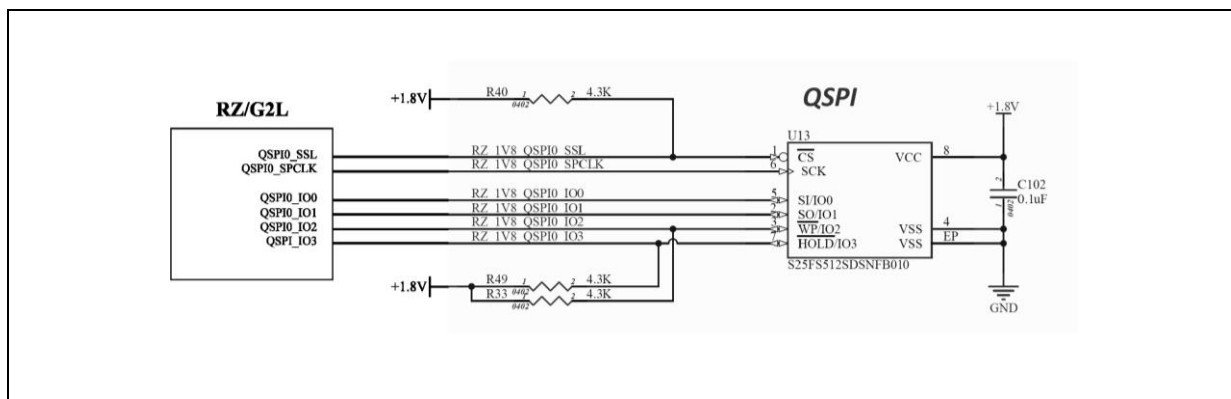
Figure 77: QSPI interface.
