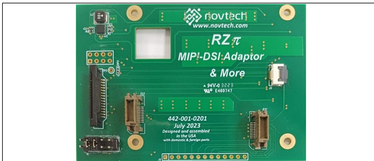
Figure 81: Adaptor board
