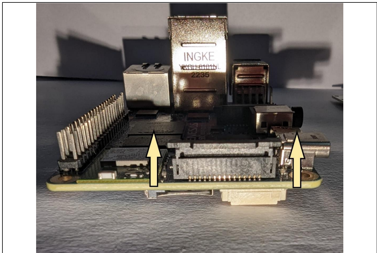
Figure 12: DSI port notch lock open by pulling it up.
