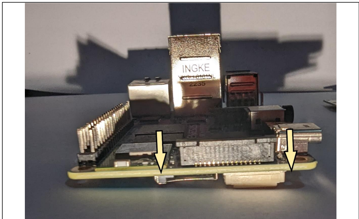
Figure 15: DSI port notch in the lock position. The cable is not shown to keep the notch in clear view.
