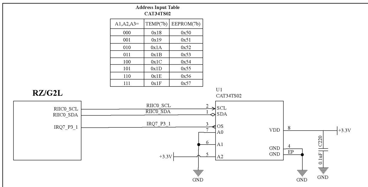
Figure 79: I2C EEPROM Block Diagram
