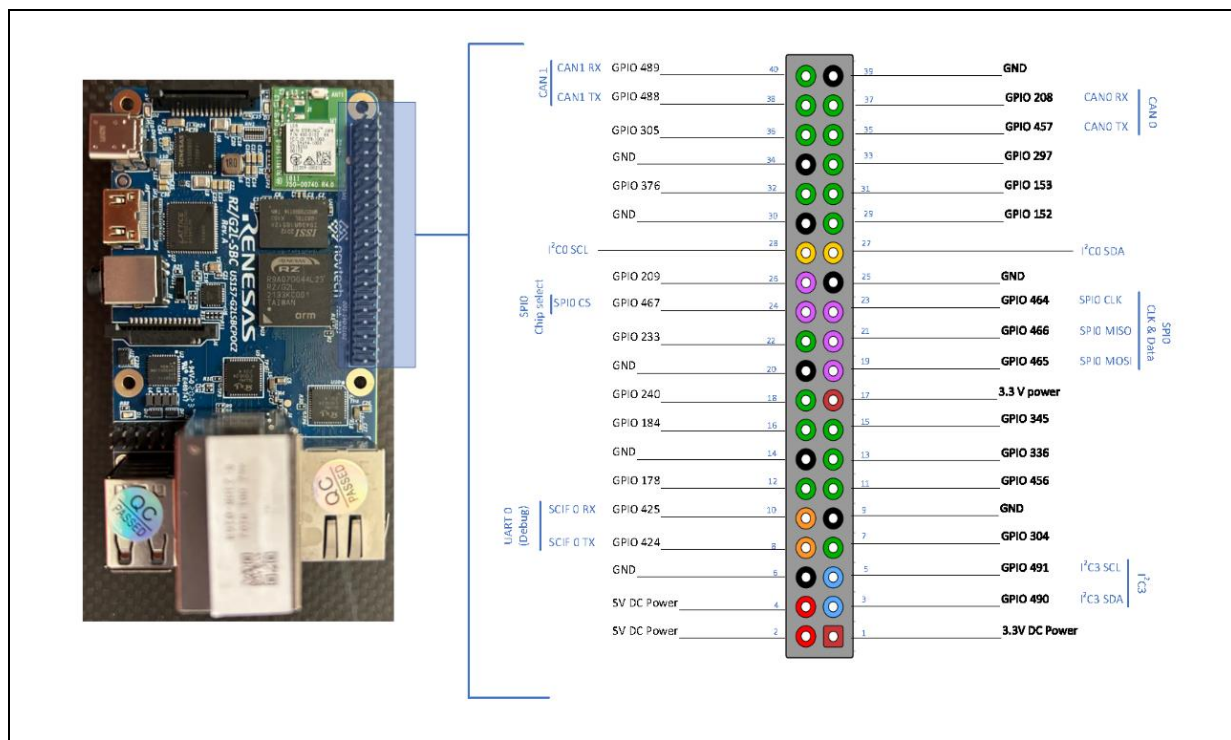
Figure 71: 40 PIN GPIO map with orientation details.
