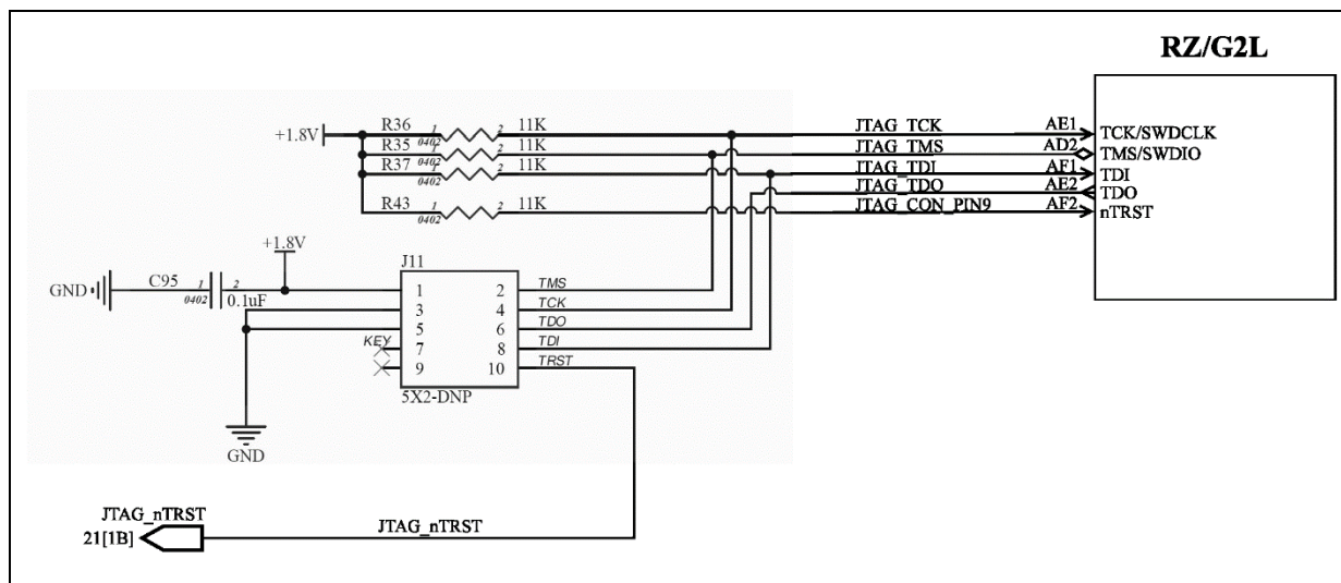
Figure 75: JTAG/SWD Block Diagram
