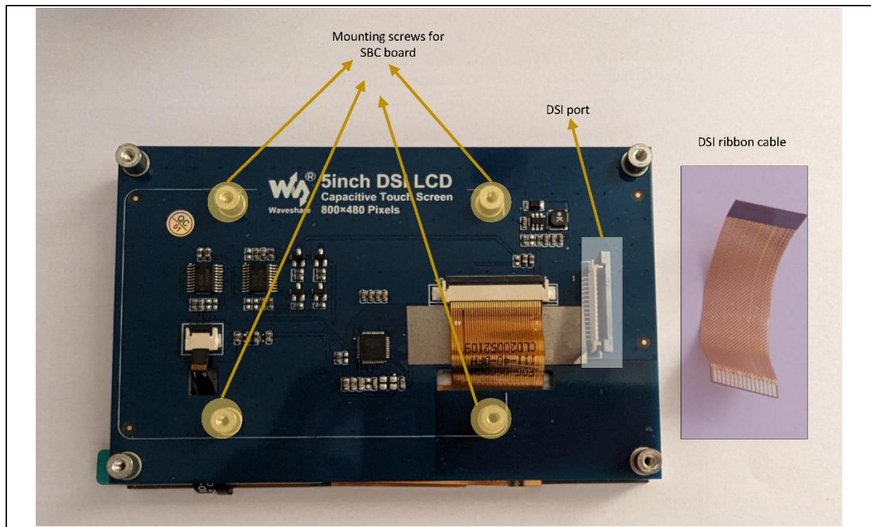
Figure 11: Waveshare 5" DSI touch panel read side picture with flat ribbon cable.
