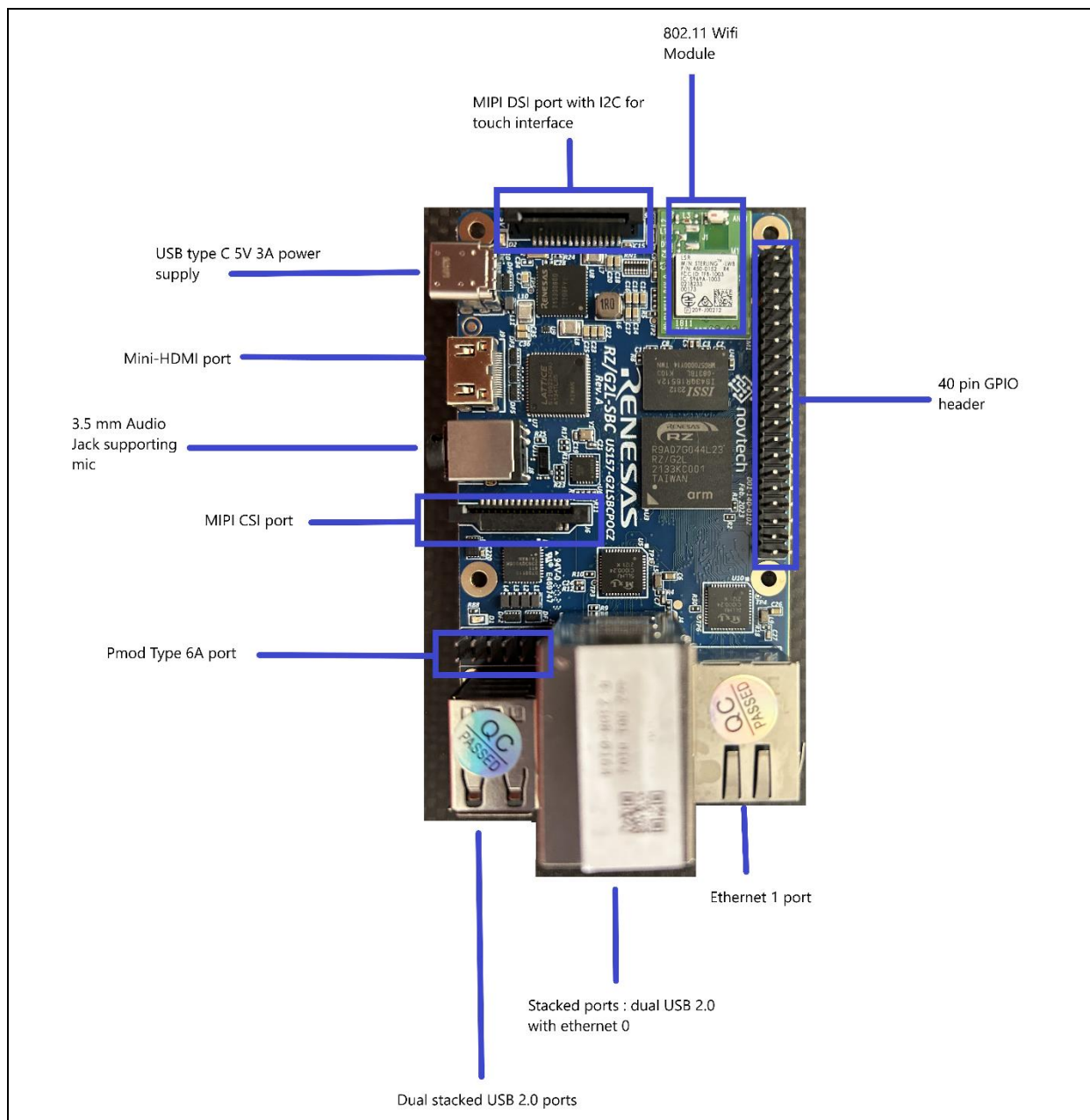
Figure 55: RZ/G2L-SBC top side connectors.
