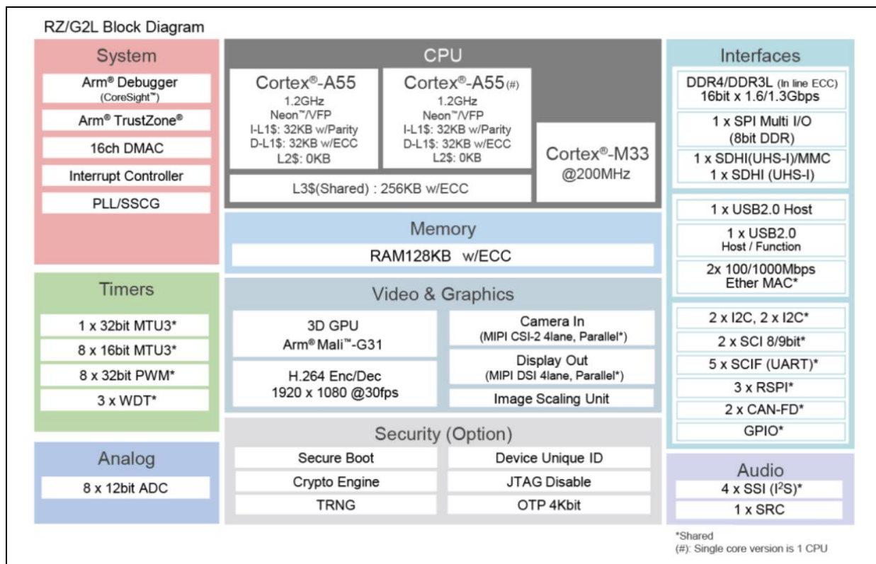
Figure 52: RZ/G2L SoC (System on Chip) Overview
