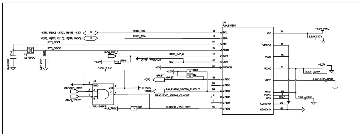
Figure 59: Block Diagram of Power Supply Regulation using RAA215300.
