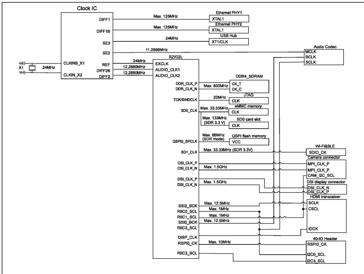
Figure 62: Block diagram of Clock interfacing.
