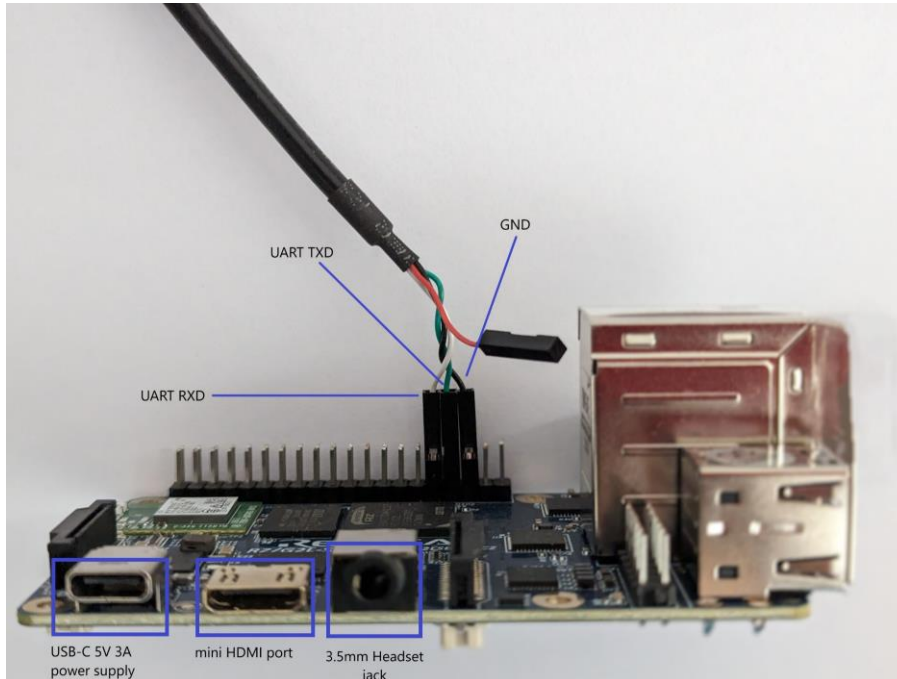
Figure 8: Cortex A55 debug UART cable interface
