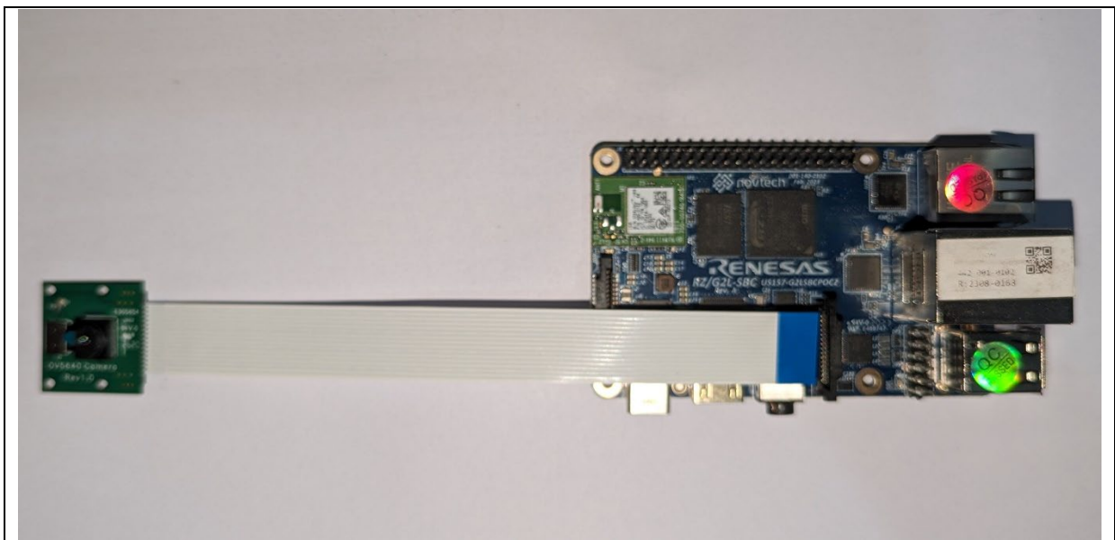
Figure 19. Orientation of the camera module. Blue stripe upward.
