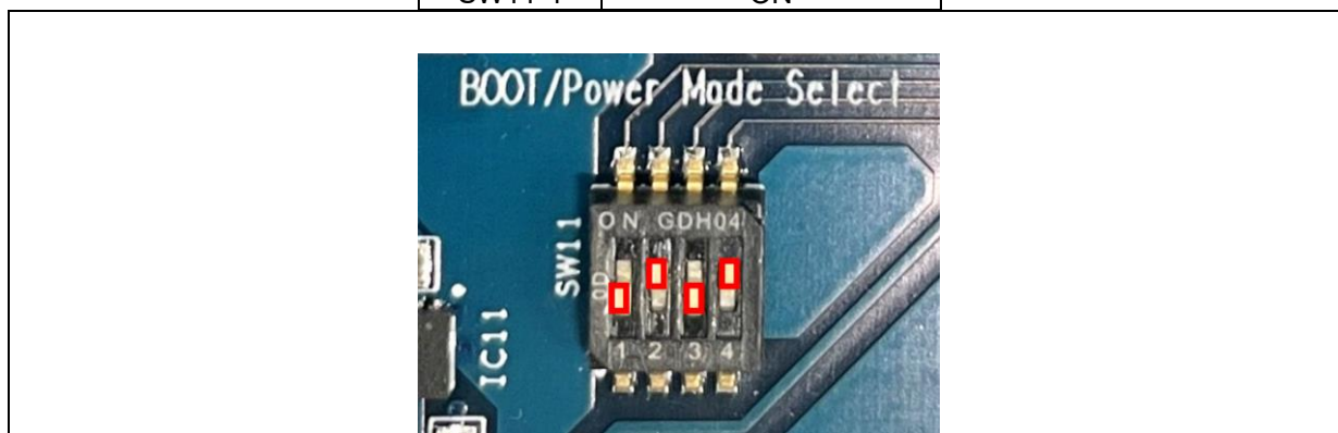
Figure 22. SW11 SCIF Download Mode - RZ/G2L-EVK & RZ/V2L-EVK
