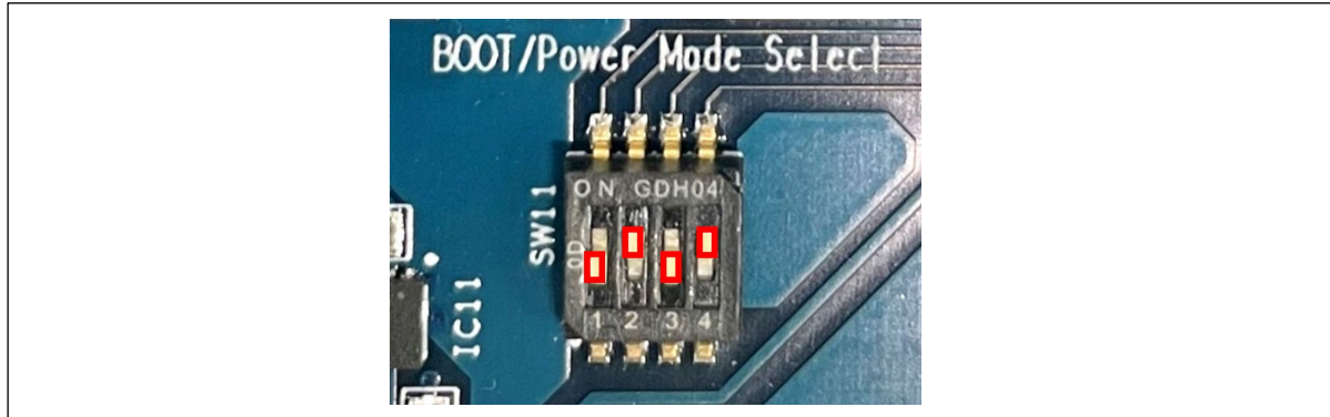
Figure 41. SW11 SCIF Download Mode - RZ/G2L-EVK & RZ/V2L-EVK
