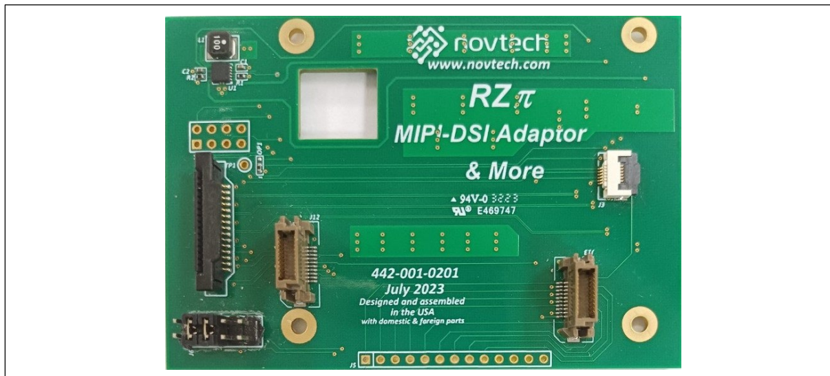
Figure 39. Adaptor board
