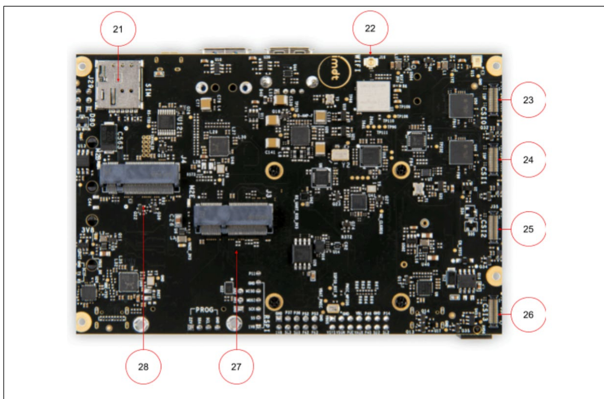
Figure 36. IMDT-V2H-SBC Bottom view
