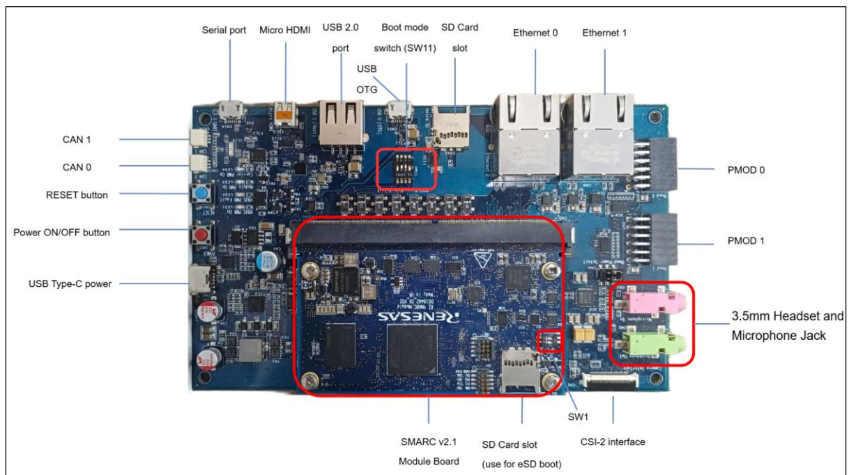
Figure 21. Overview of Connectors - RZ/G2L-EVK & RZ/V2L-EVK
