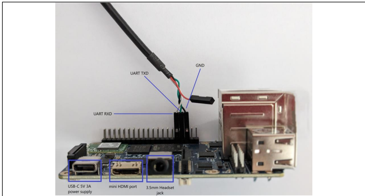
Figure 12. Cortex A55 debug UART cable interface
