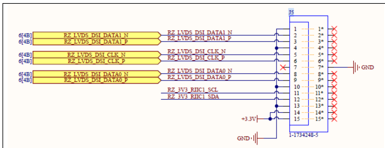
Figure 91. DSI Schematic
