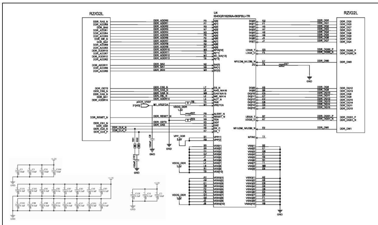
Figure 101. DDR4 SDRAM Interface
