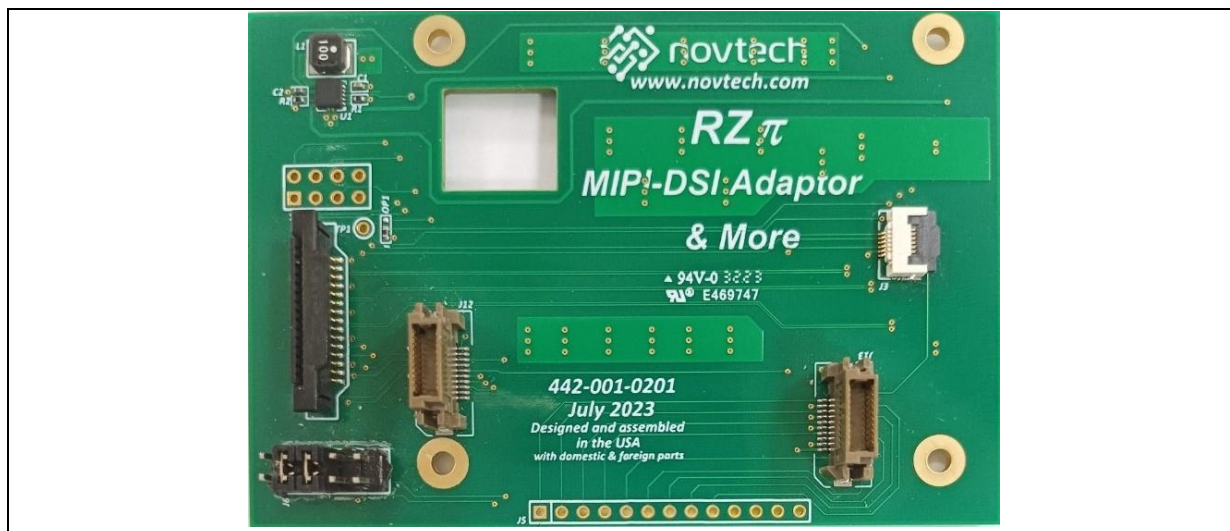
Figure 104. Adapter board
