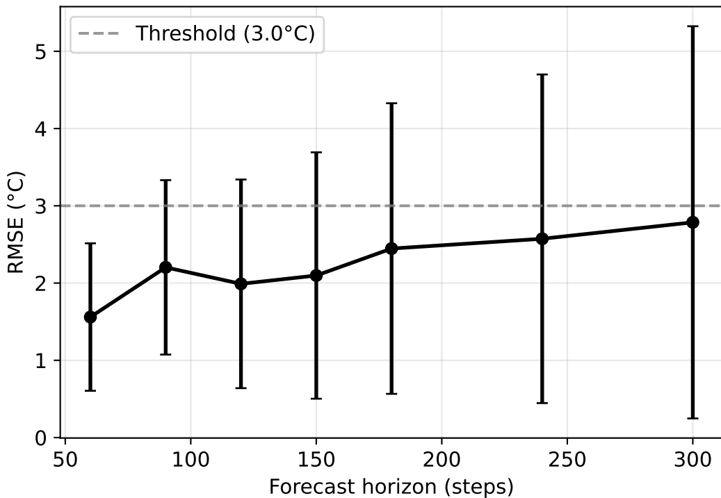
RMSE vs Horizon
