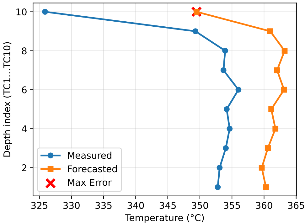
Hotspot example ( t \approx 1 s)
