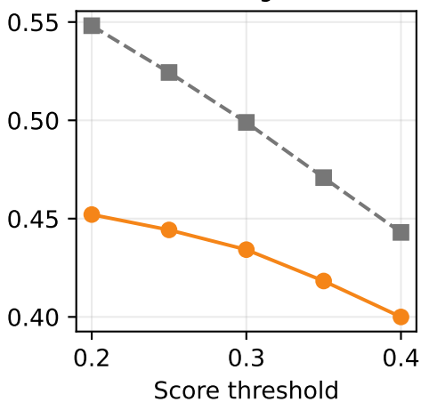
Grounding DINO
