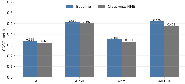
Fig. 5. OWL-ViT on the 100-image diagnostic subset before and after class-wise NMS.
