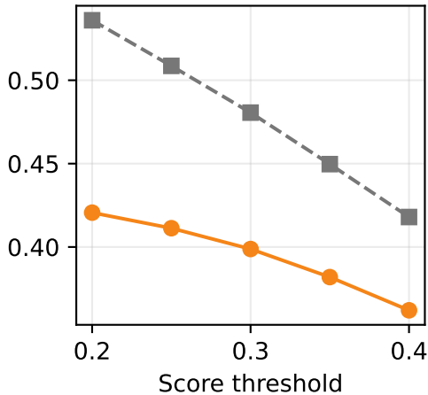
Grounding DINO
