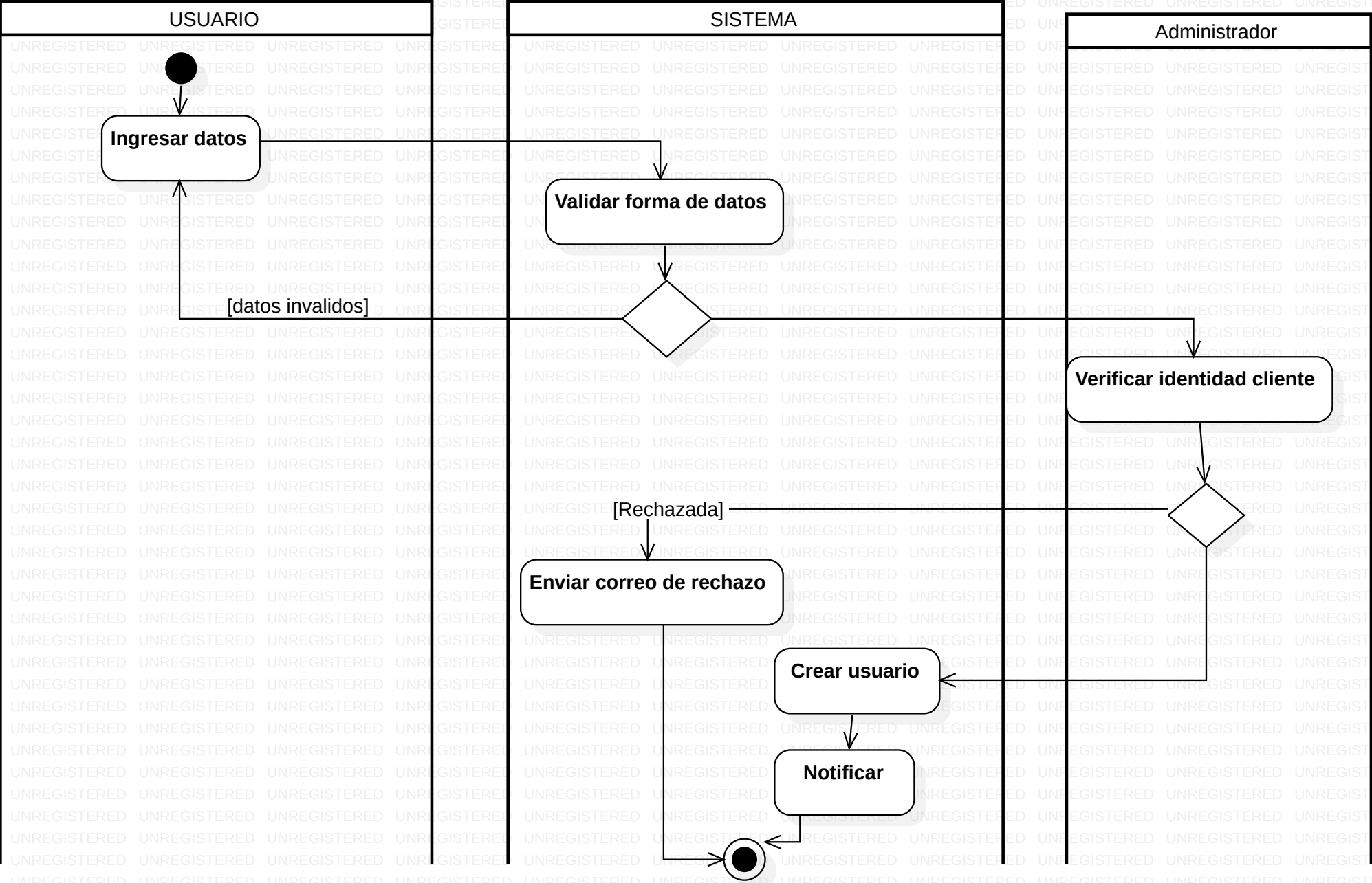
Activity1::ActivityDiagram1
