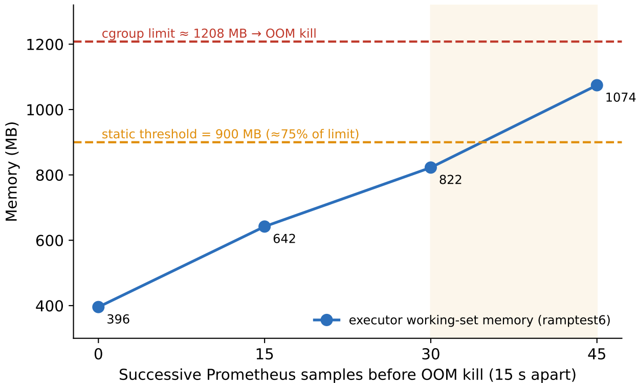
Figure 3. executor_oom gradual ramp gives the static threshold a real lead time (mean 64.9 s, 48-83 s across 8 reps)
