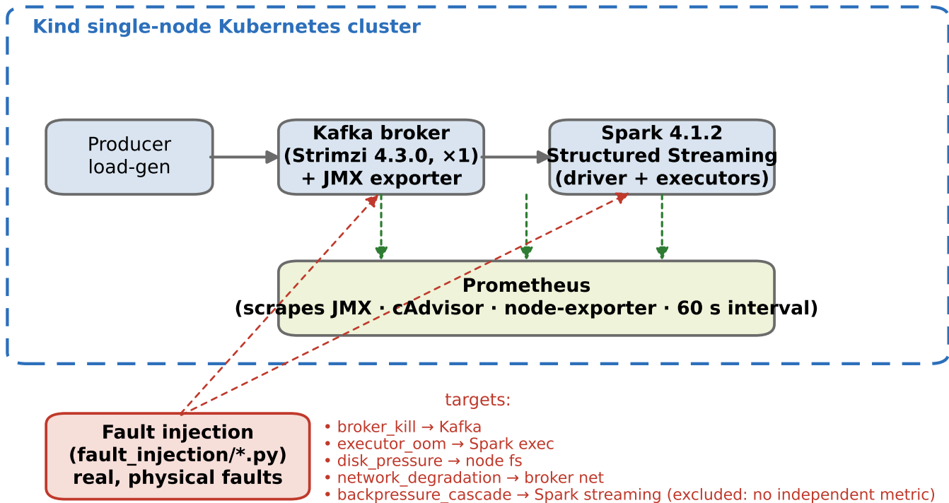
Figure 2. System under test and fault-injection points
