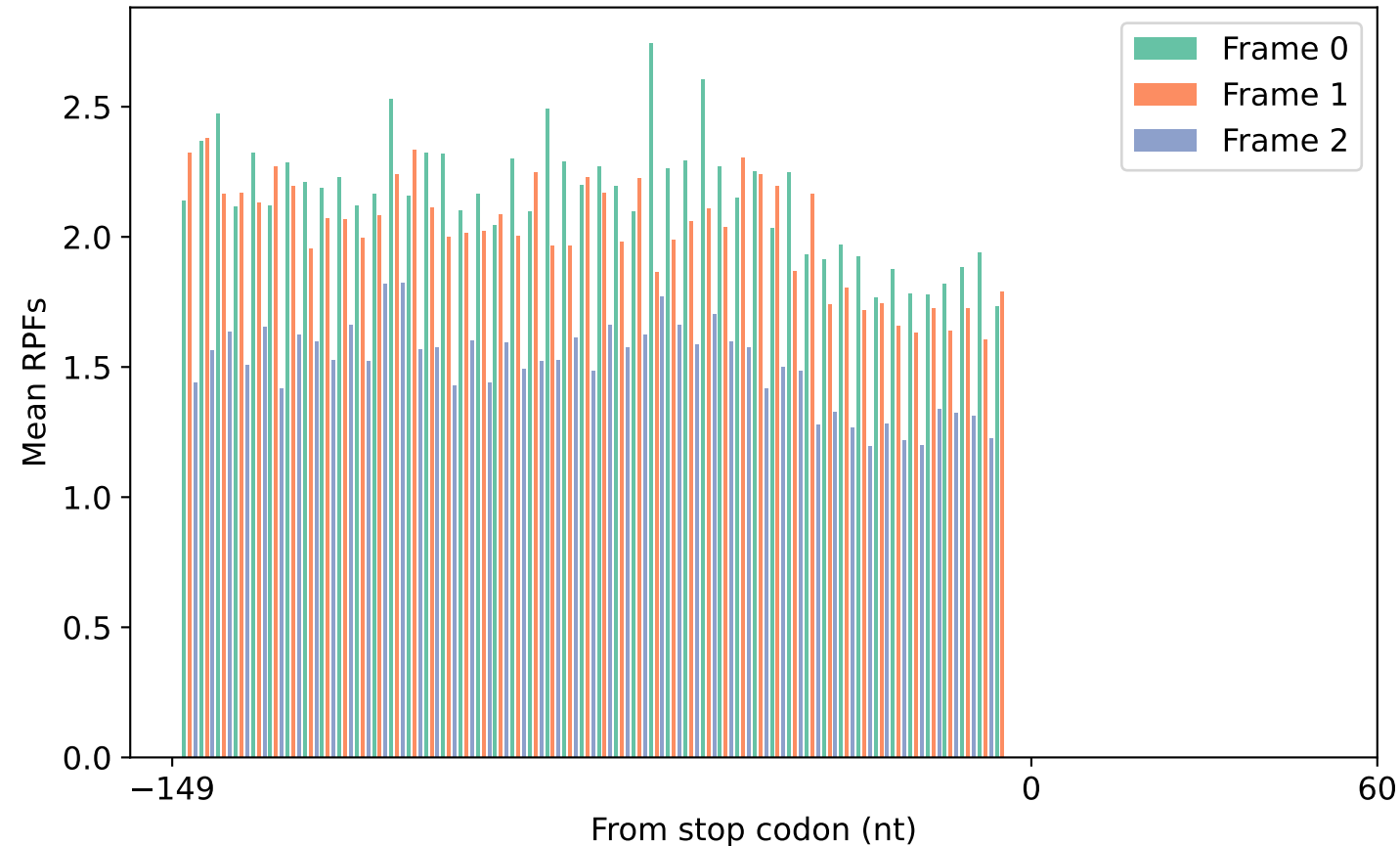
Mean RPFs of TTS region (5206 genes)
