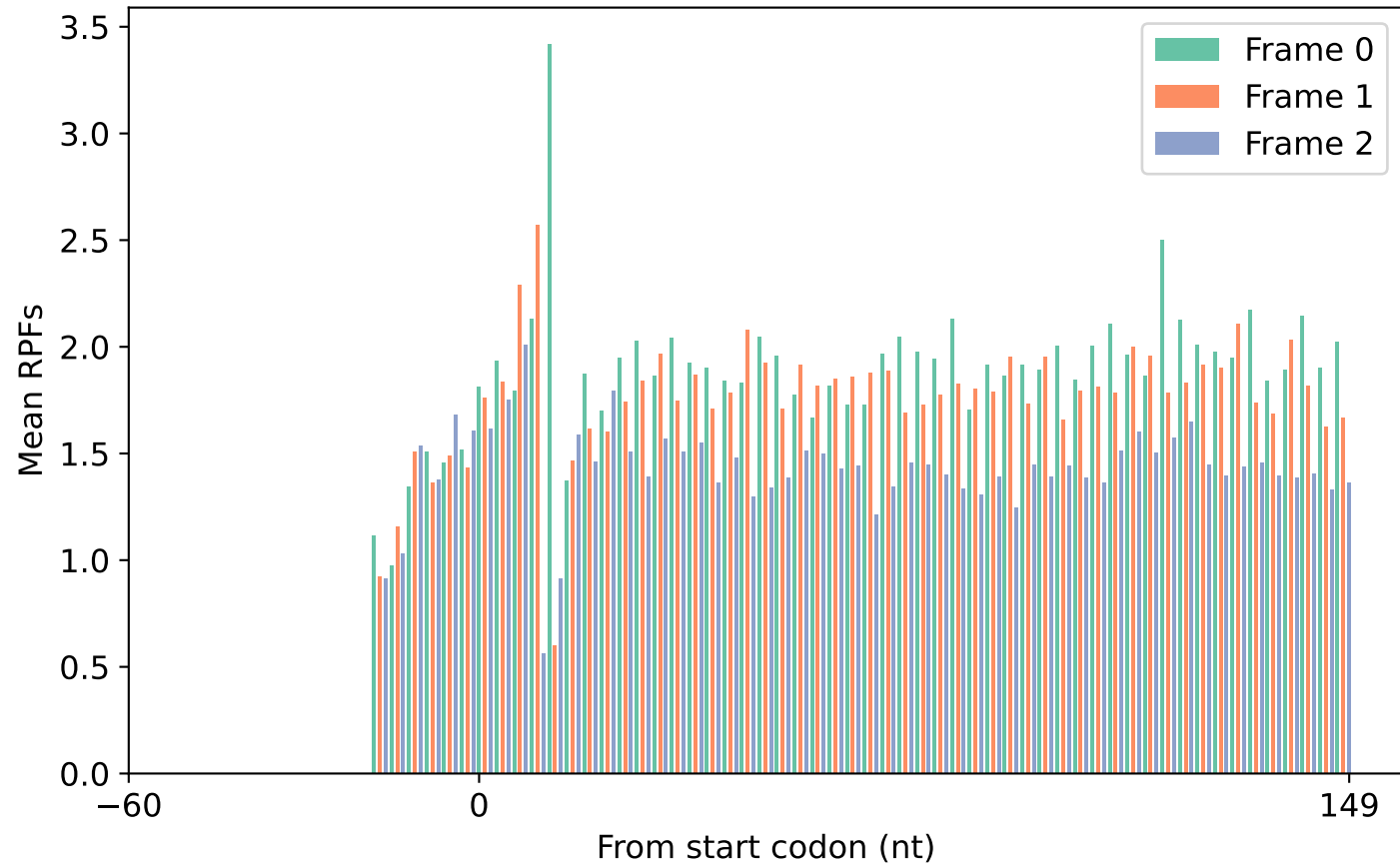
Mean RPFs of TIS region (5206 genes)
