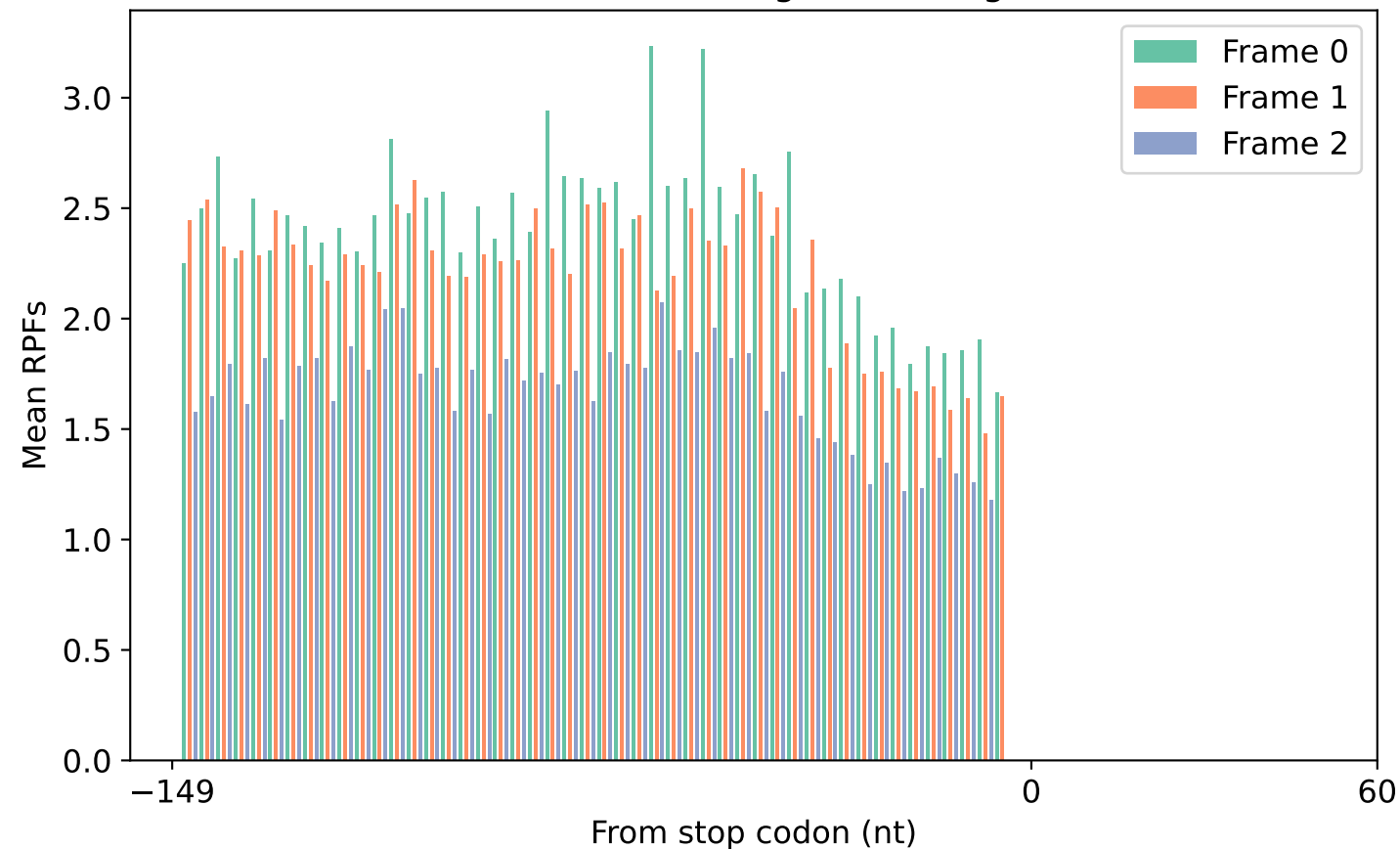
Mean RPFs of TTS region (5197 genes)
