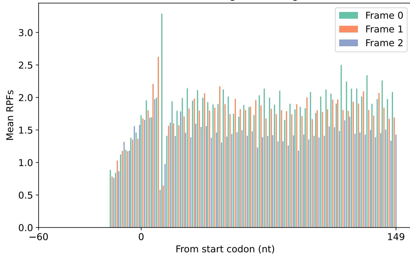
Mean RPFs of TIS region (5197 genes)
