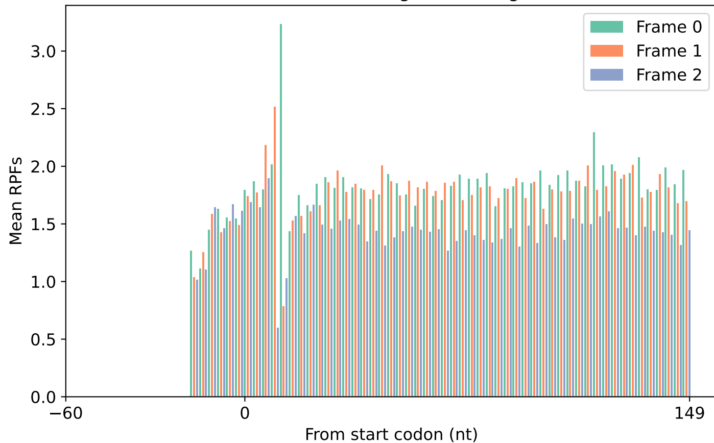
Mean RPFs of TIS region (5248 genes)
