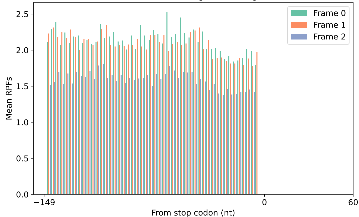
Mean RPFs of TTS region (5248 genes)
