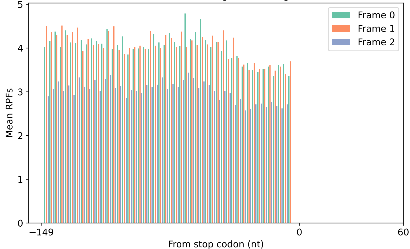
Mean RPFs of TTS region (5354 genes)
