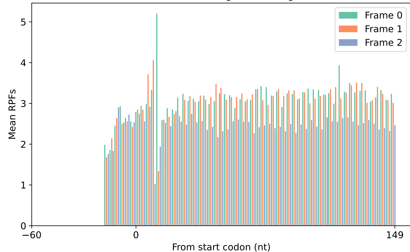
Mean RPFs of TIS region (5354 genes)
