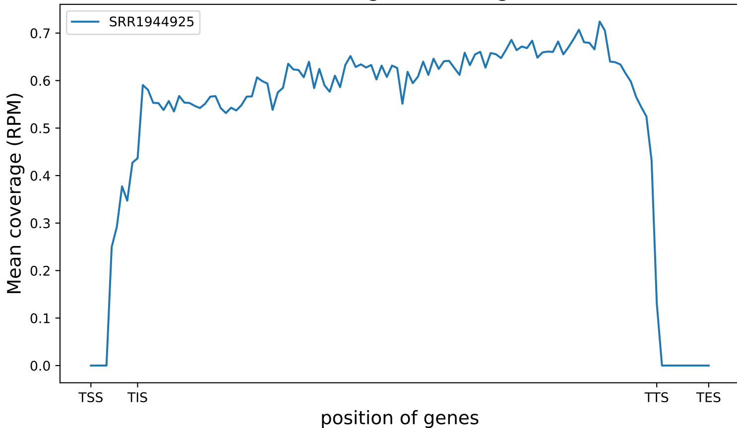
Mean coverage of (5287 genes)
