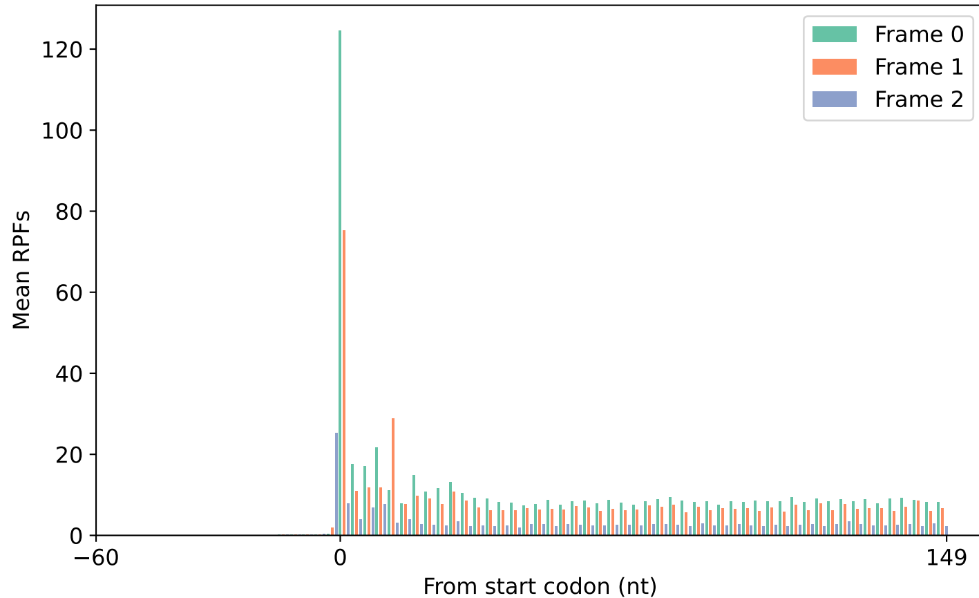
Mean RPFs of TIS region (5074 genes)
