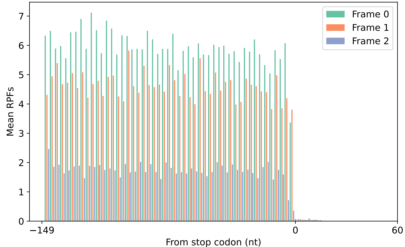
Mean RPFs of TTS region (5074 genes)
