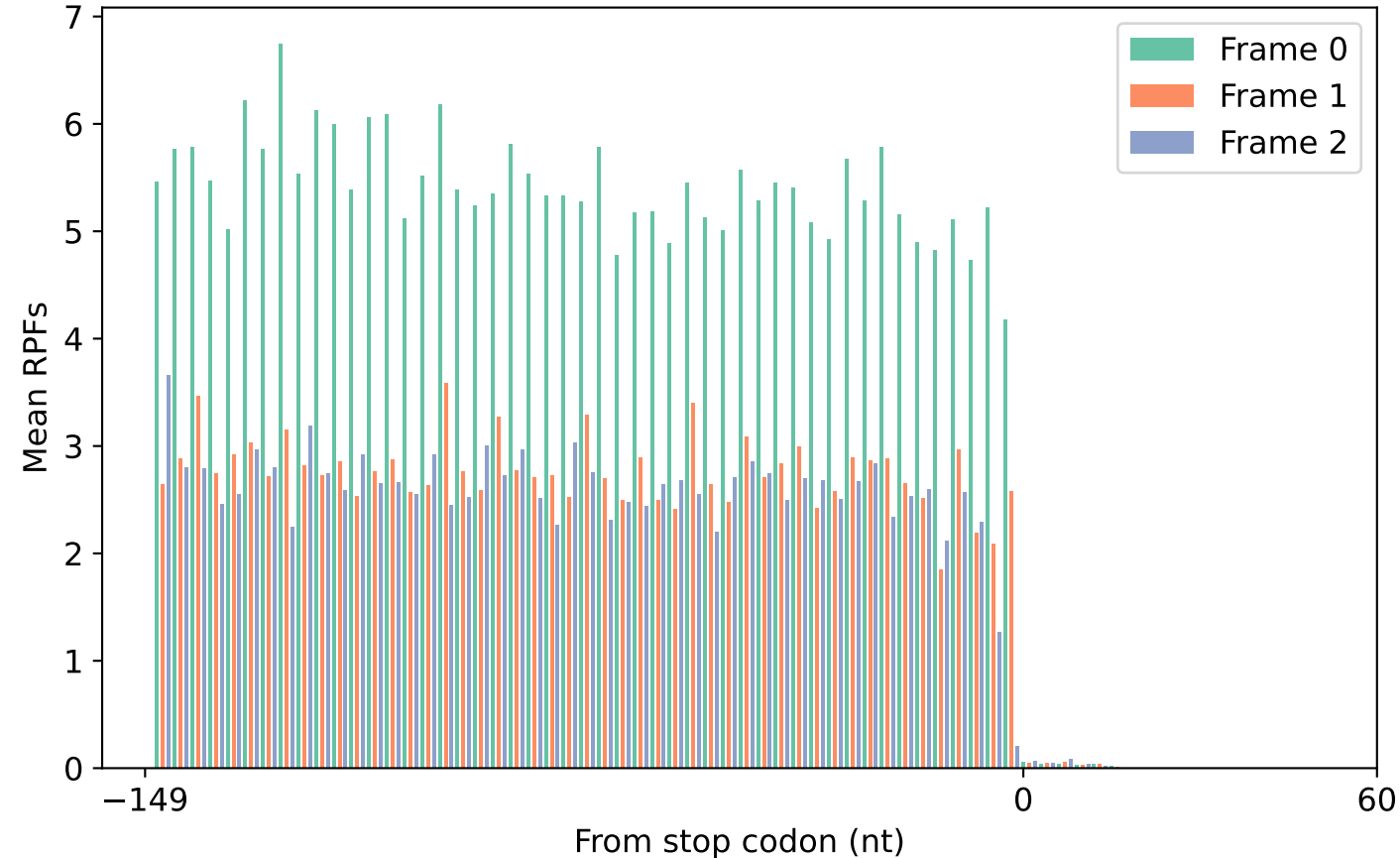
Mean RPFs of TTS region (5036 genes)
