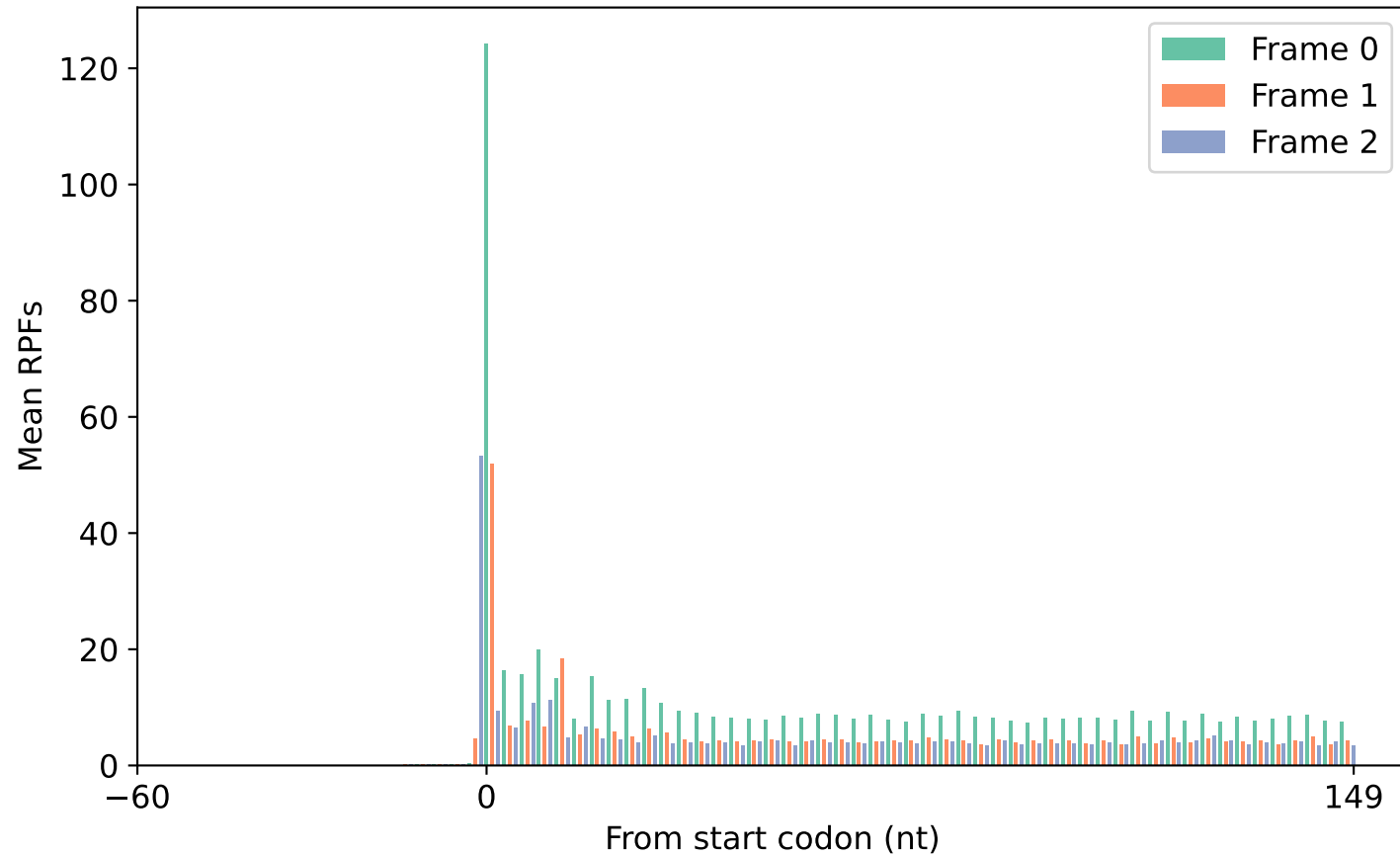
Mean RPFs of TIS region (5036 genes)
