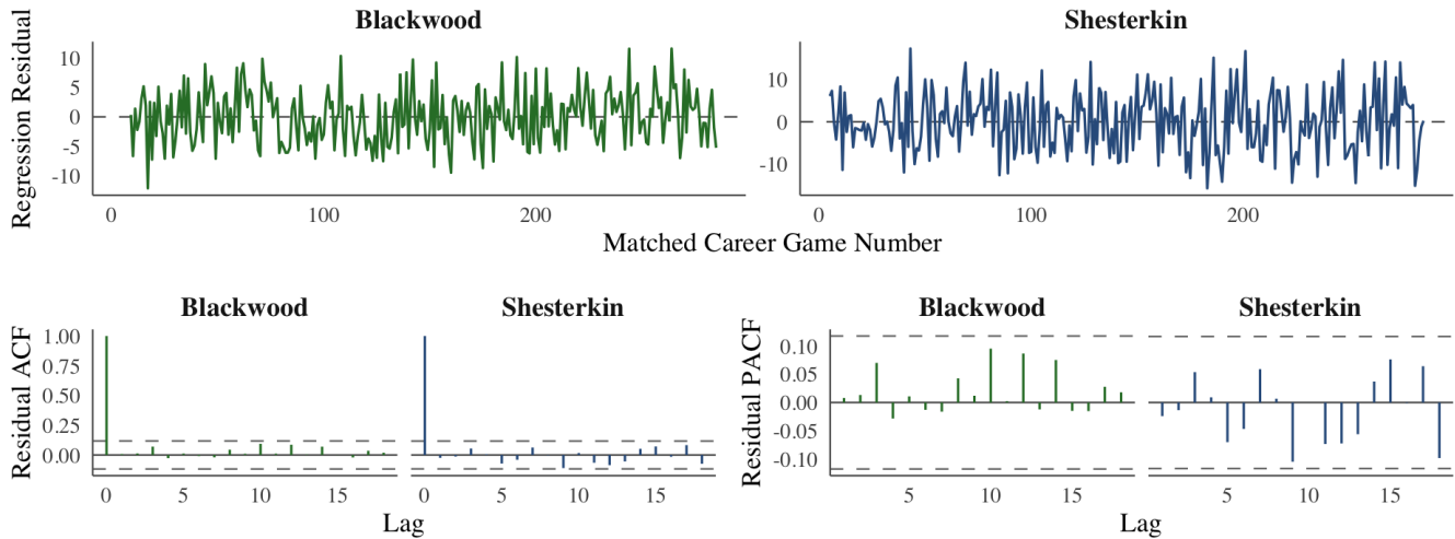
Figure 2: Residual index plots, residual ACF, and residual PACF after the transformed lagged regressions.
