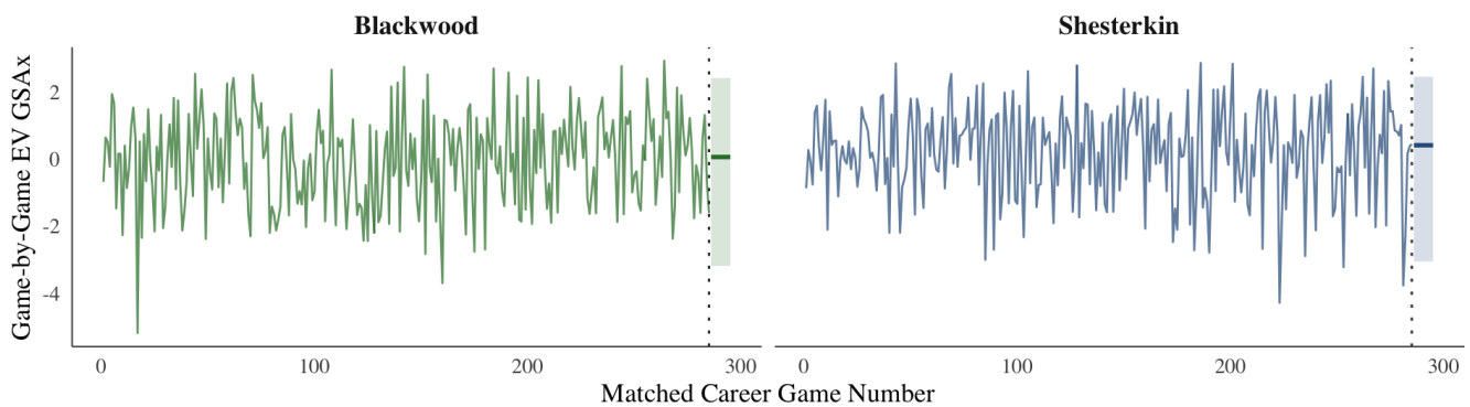
Figure 3: Ten-game response forecasts from the final manual model under average future predictor conditions. The dotted line marks the last observed matched game.
