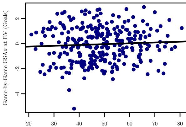
Blackwood: GSAX vs Lagged Team xGF% (Lead 5)
