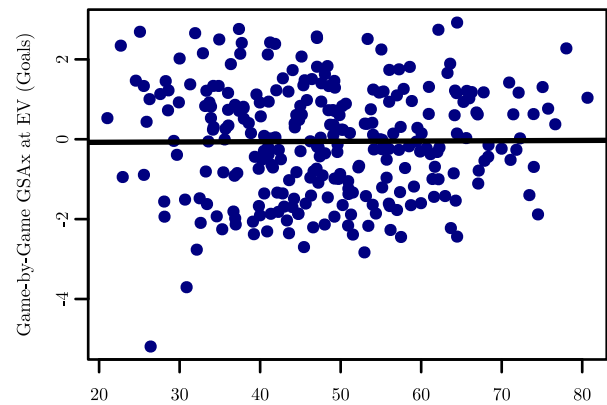
Blackwood: GSAX vs Lagged Team xGF% (Lead 6)
