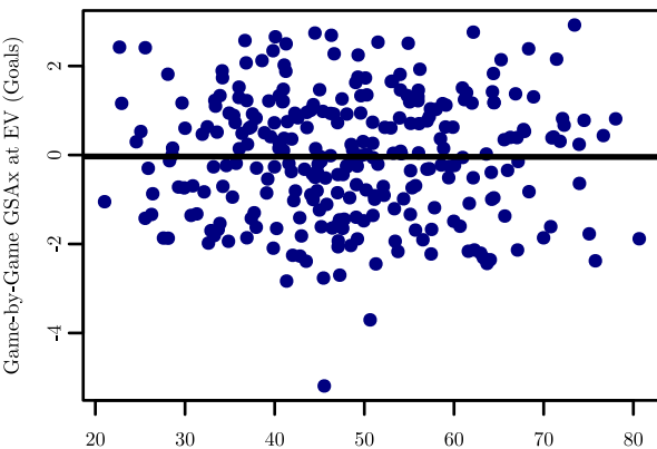
Blackwood: GSAX vs Lagged Team xGF% (Lead 1)
