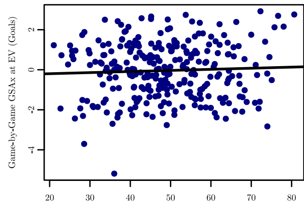
Blackwood: GSAX vs Lagged Team xGF% (Lead 3)
