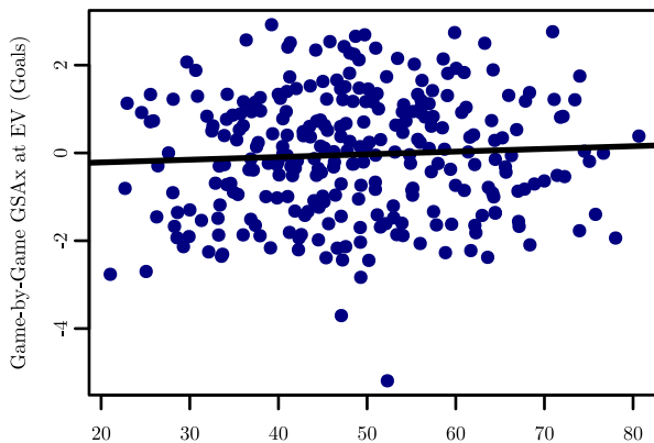
Blackwood: GSAX vs Lagged Team xGF% (Lead 2)
