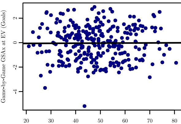
Blackwood: GSAX vs Lagged Team xGF% (Lead 4)
