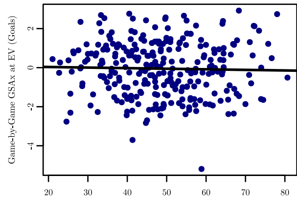
Blackwood: GSAX vs Lagged Team xGF% (Lead 9)
