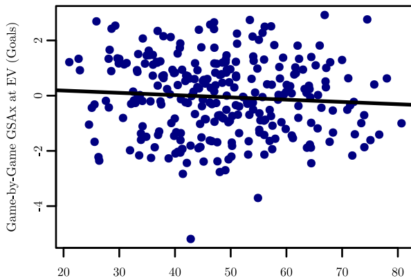
Blackwood: GSAX vs Lagged Team xGF% (Lead 8)
