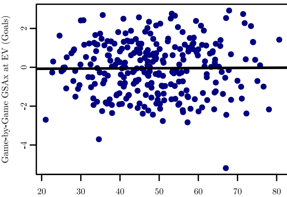
Blackwood: GSAX vs Lagged Team xGF% (Lead 7)
