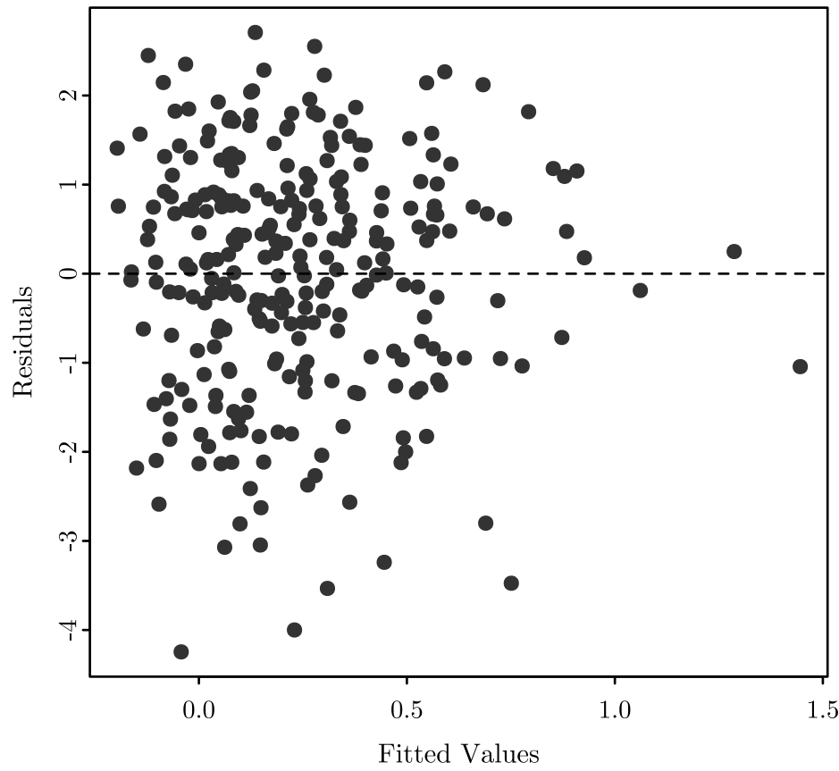
Shesterkin: Residuals vs Fitted
