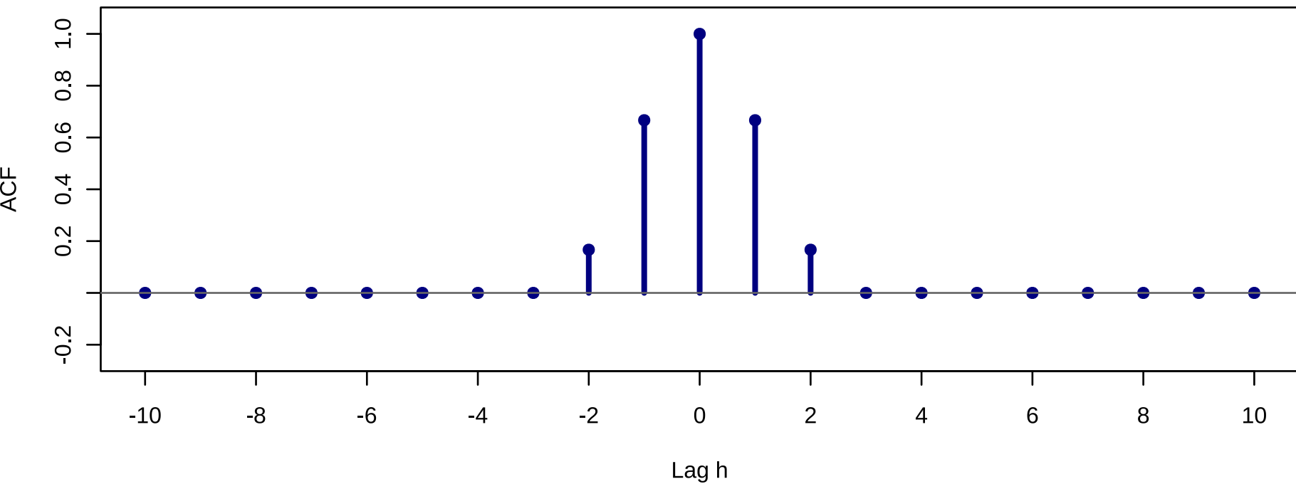
Problem 2: ACF
