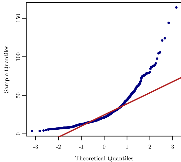
QQ Plot of Original Varves
