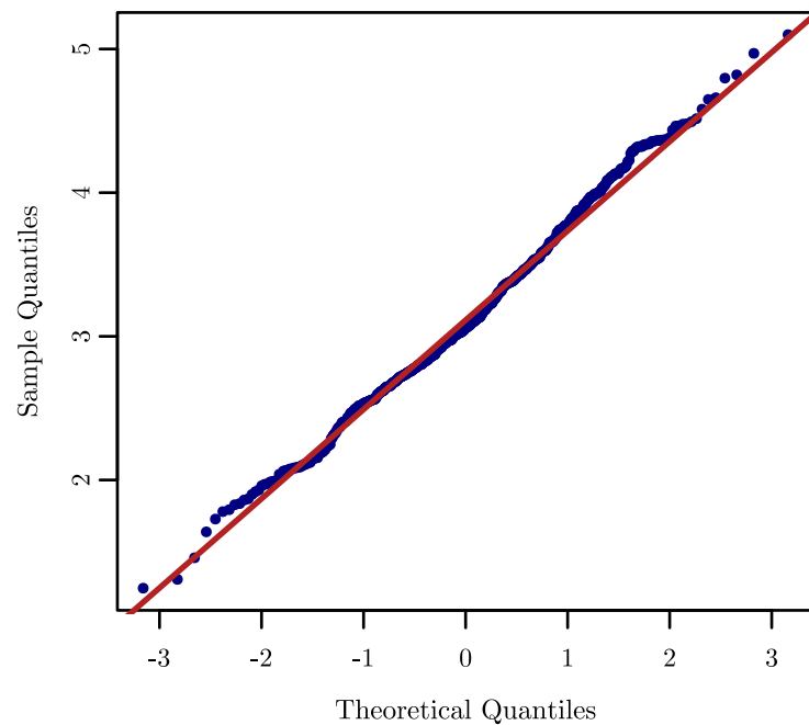
QQ Plot of Logged Varves
