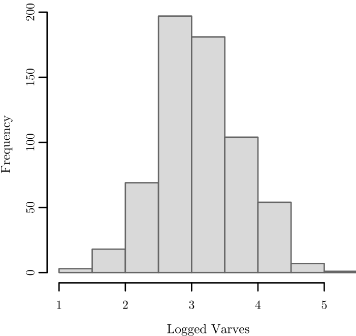
Histogram of Logged Varves
