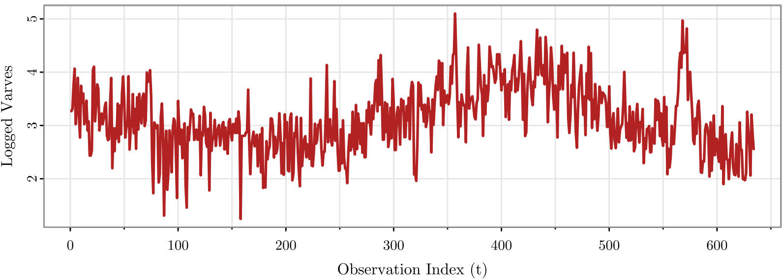
Glacial Varves: Log-Transformed Series
