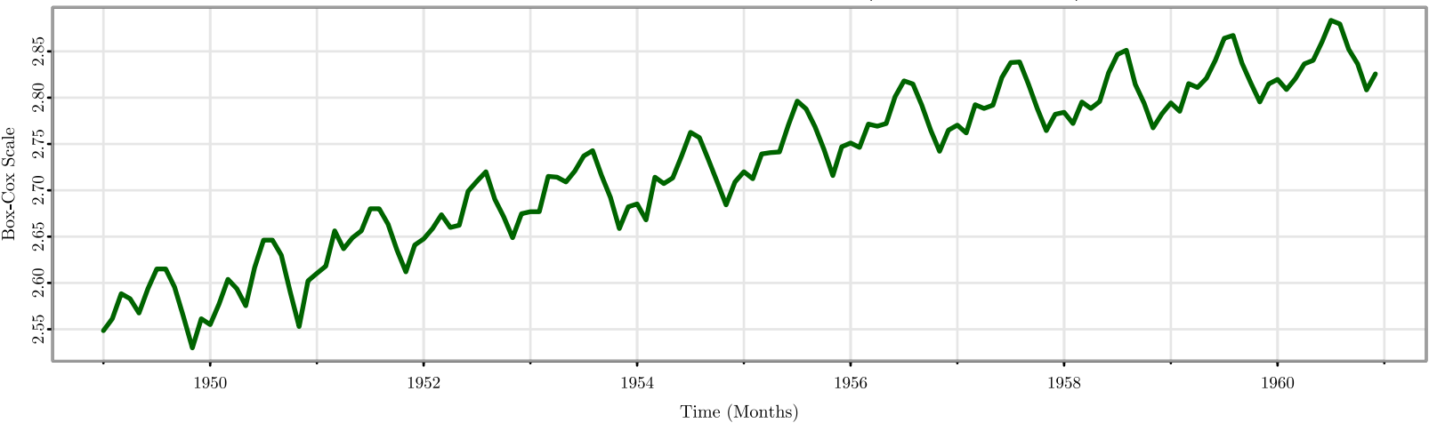
AirPassengers: Box-Cox Transformation (lambda = -0.2947)
