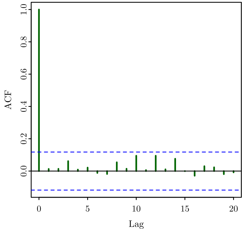
Blackwood: Final Response ACF
