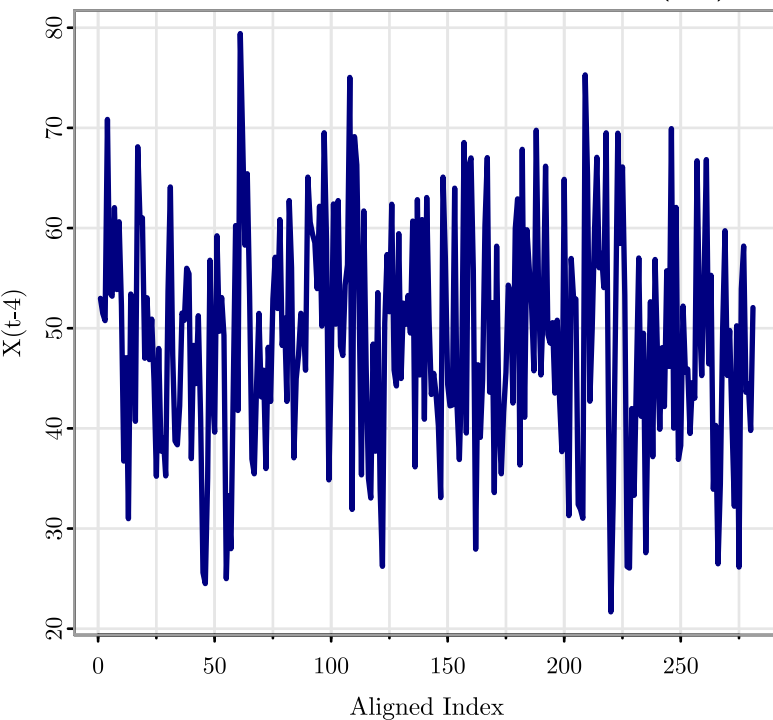
Shesterkin: Lagged Team xGF% (t-4)
