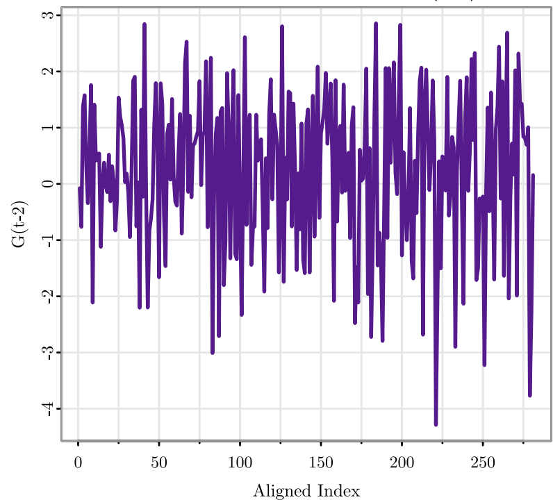
Shesterkin: Lagged GSAX (t-2)
