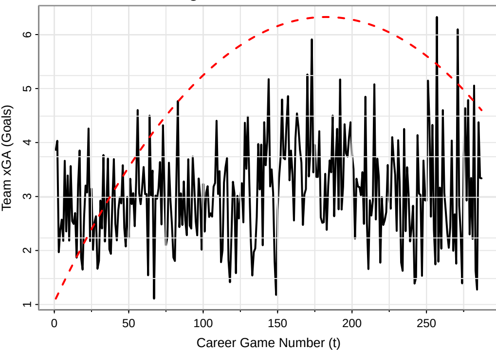
team_xga: Observed vs Selected Fit
