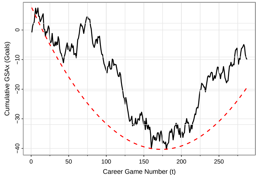
shots_against: Observed vs Selected Fit
