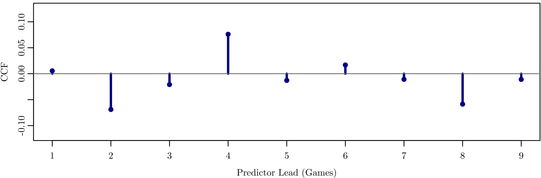
Shesterkin: Lead CCF of Team xGF% and GSAx
