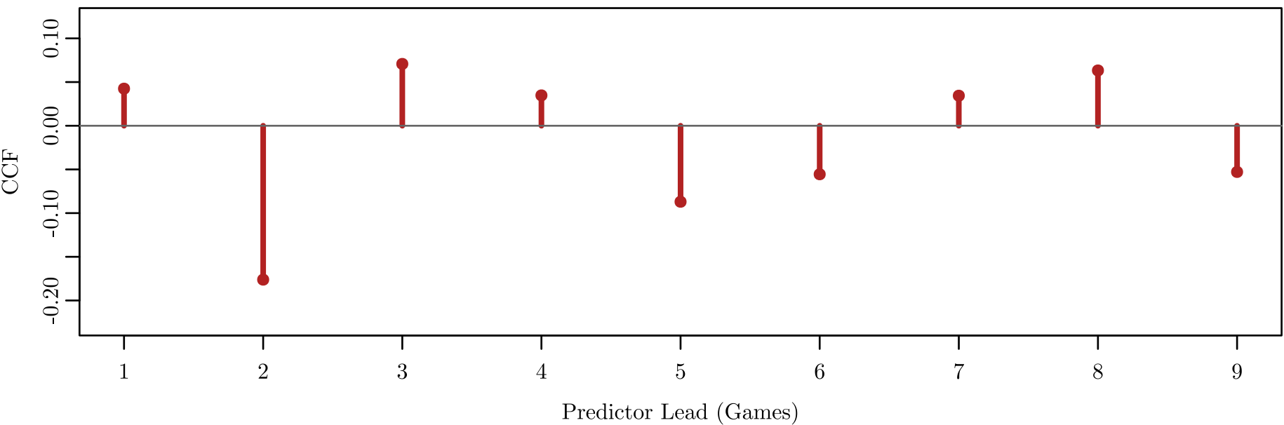
Shesterkin: Lead CCF of Save Percentage and GSAx
