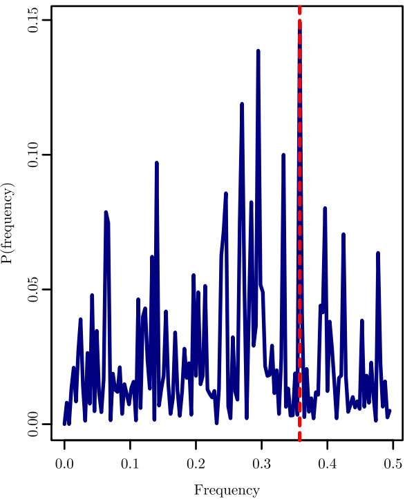
Shesterkin Detrended: GSAX
