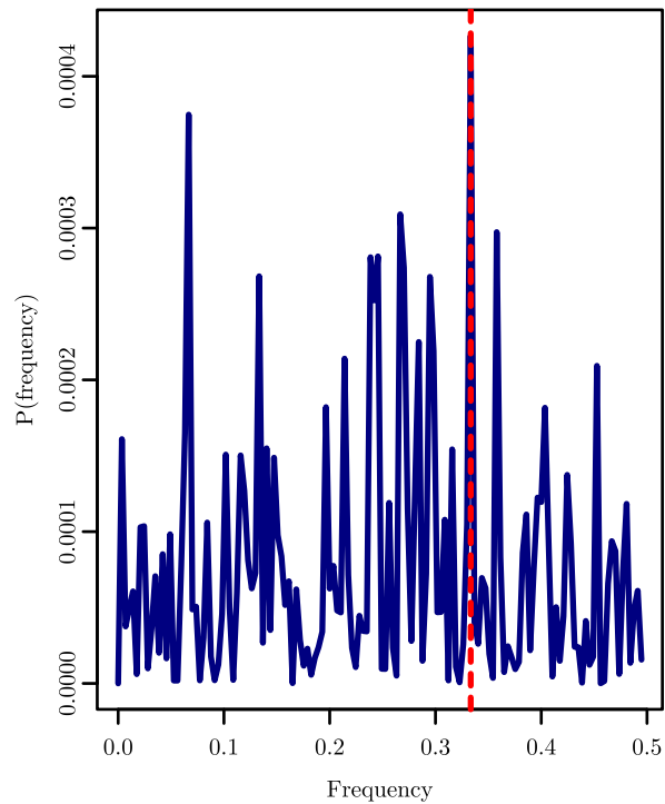
Shesterkin Detrended: Save Percentage
