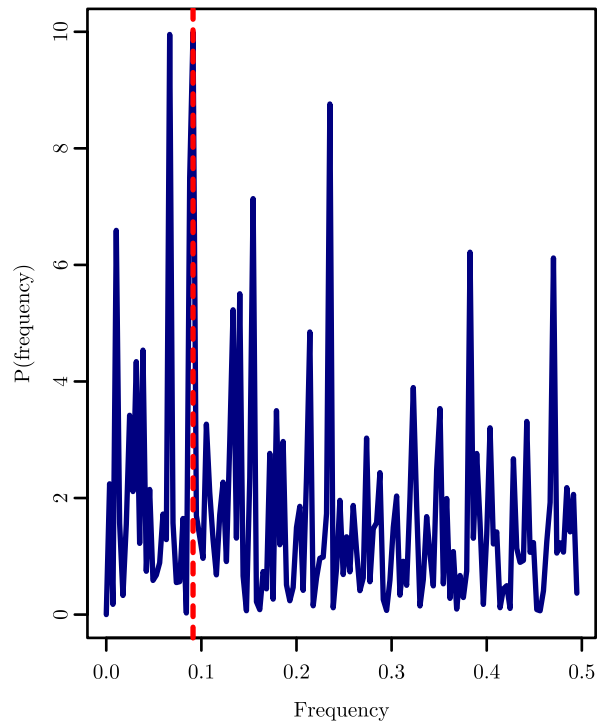
Shesterkin Detrended: Team xGF%
