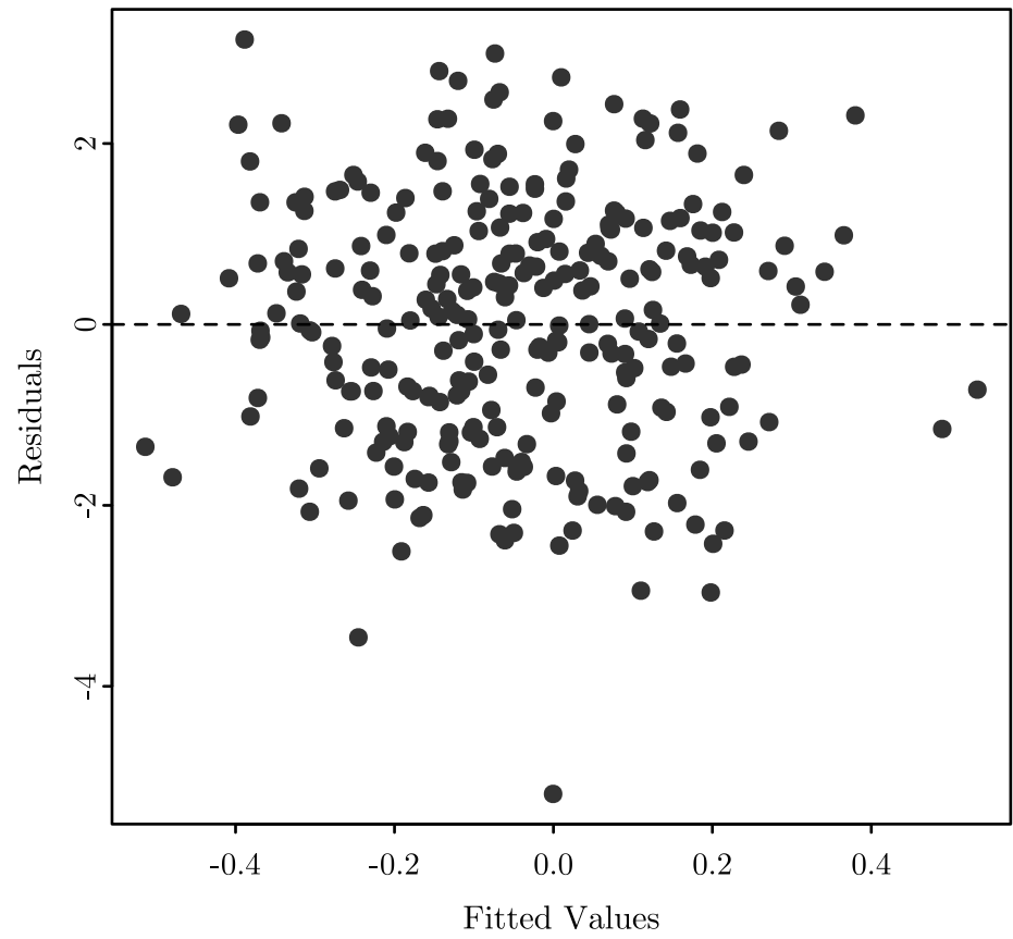
Blackwood: Residuals vs Fitted
