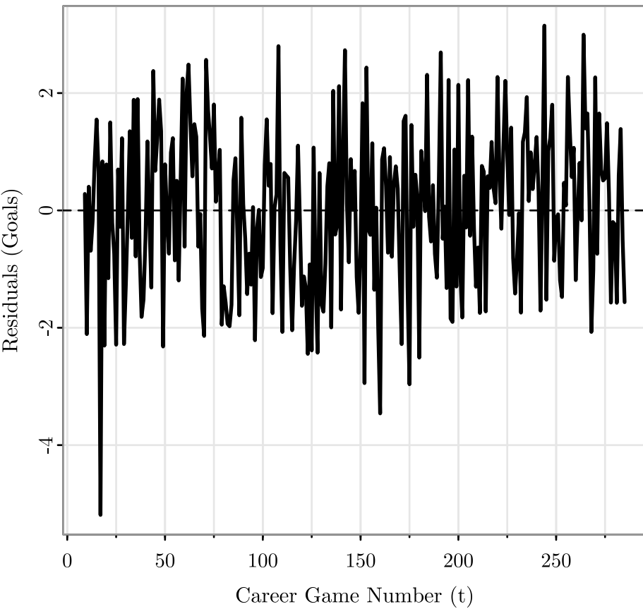
Blackwood: Residuals from Lagged Regression
