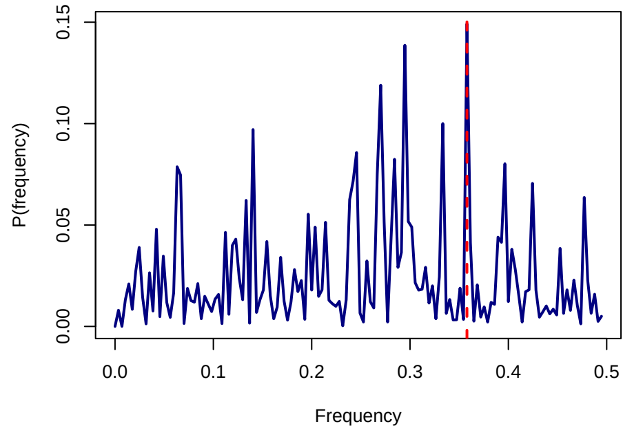
Shesterkin: Periodogram for gsax_ev
