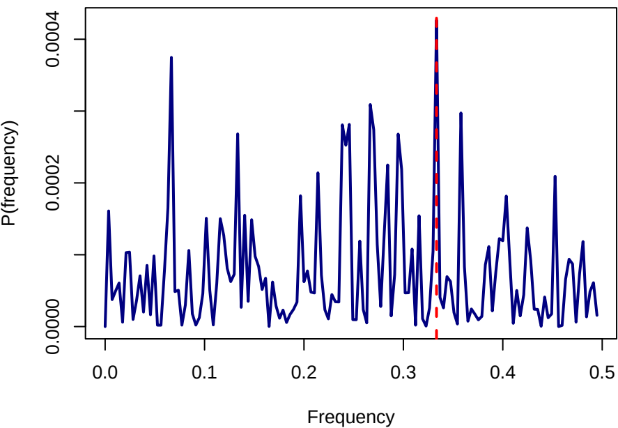
Shesterkin: Periodogram for sv_pct_ev
