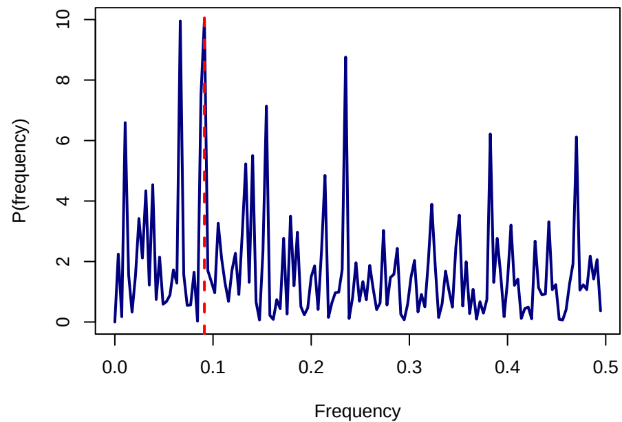
Shesterkin: Periodogram for team_xg_pct_ev
