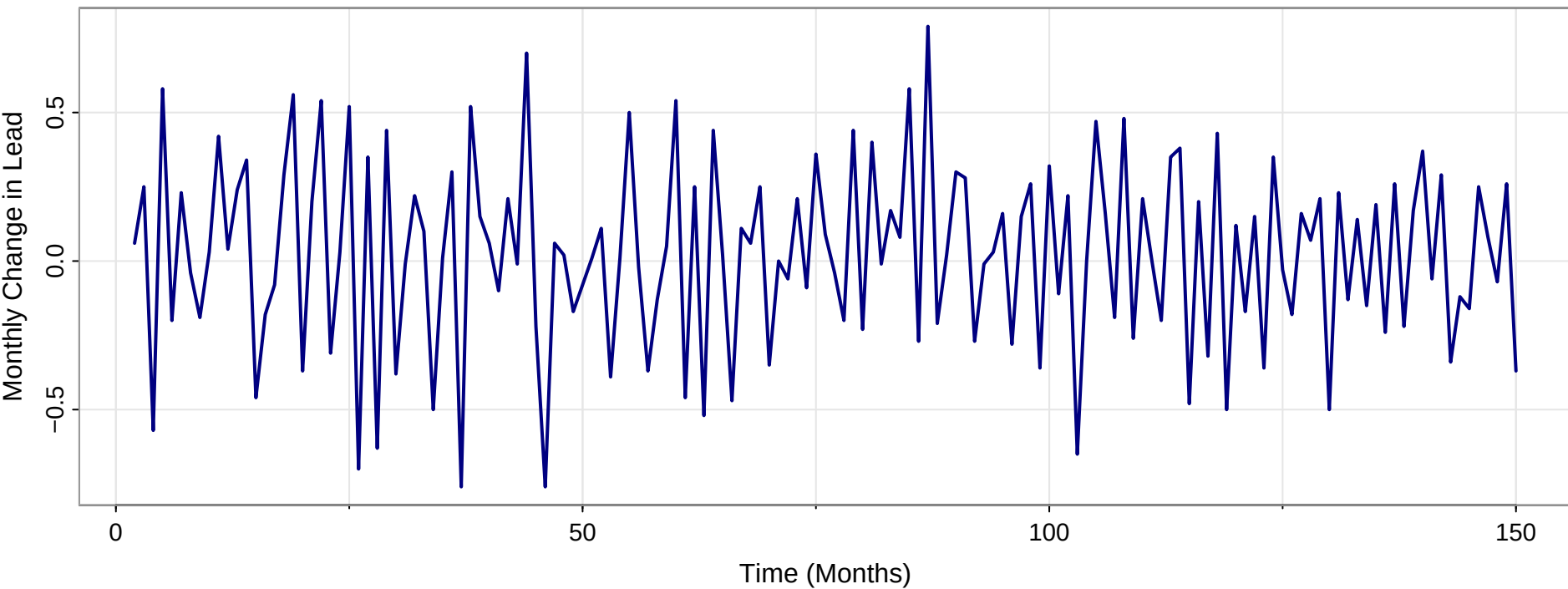
First Difference of Leading Indicator
