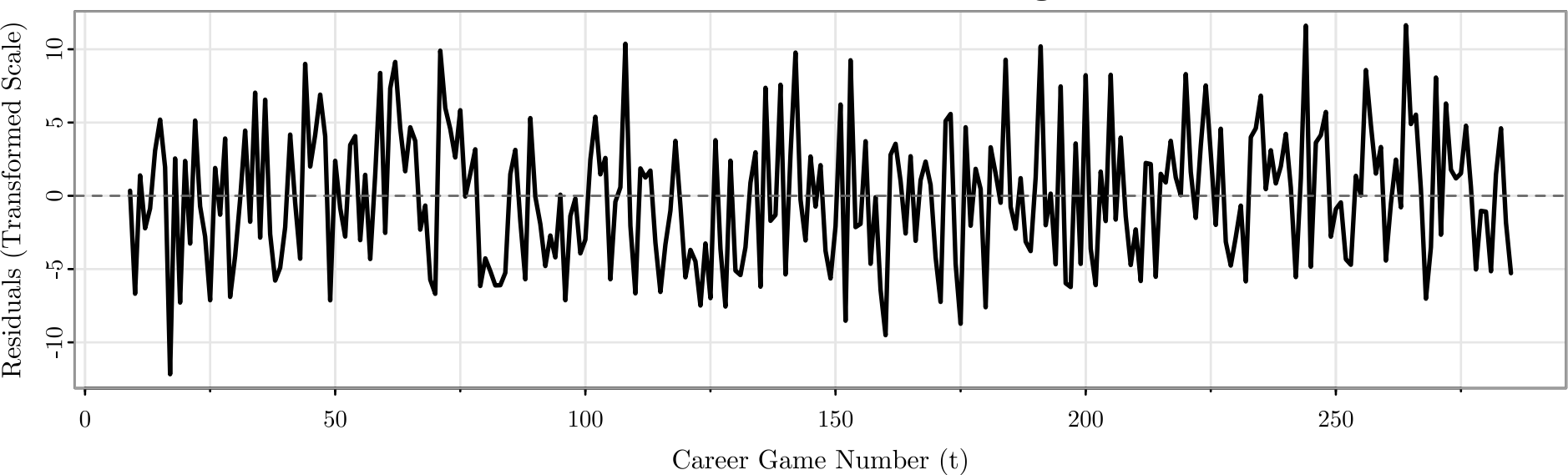
Shesterkin: Residuals from TS Regression
