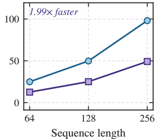
Latency, batch 32
