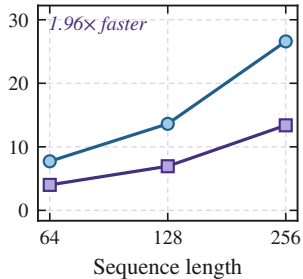
Latency, batch 8
