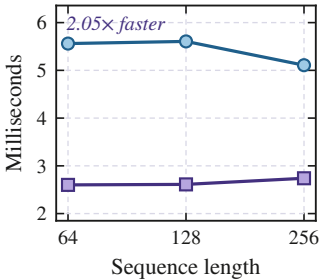
Latency, batch 1
