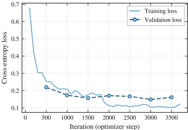
BERT-base on SST-2
