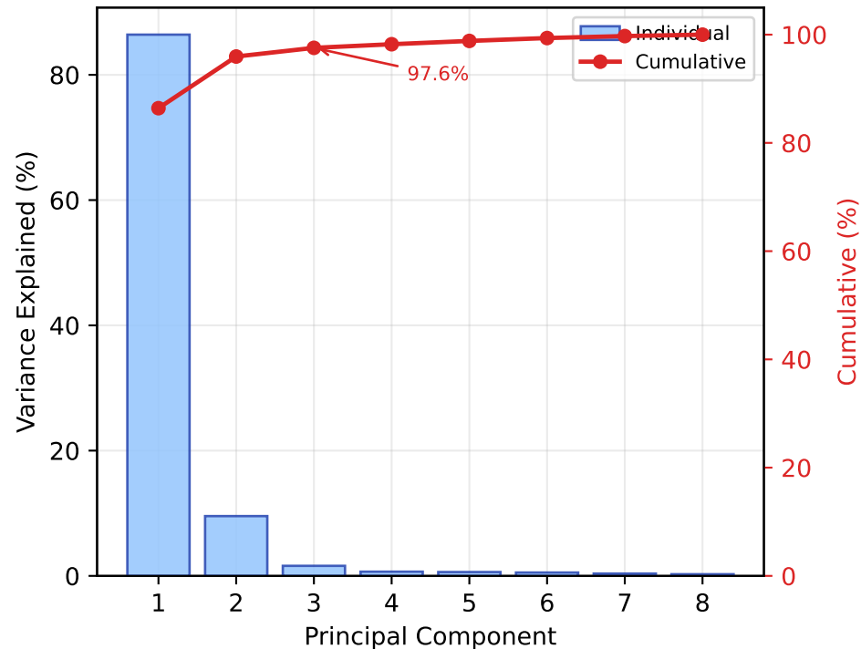
Scree Plot
