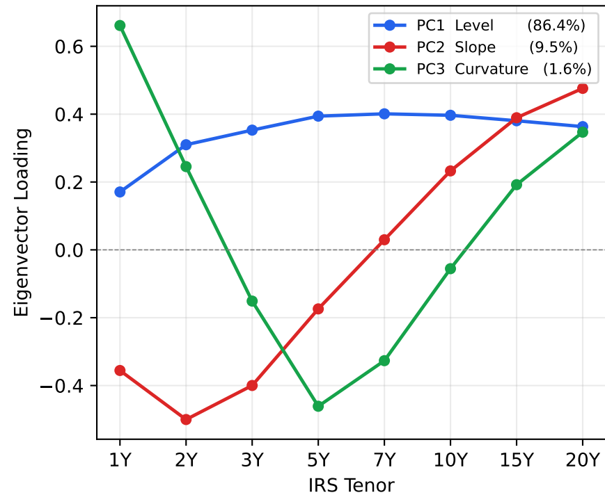
Factor Loadings
