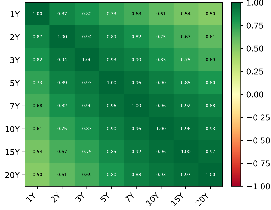
Rate-Change Correlations
