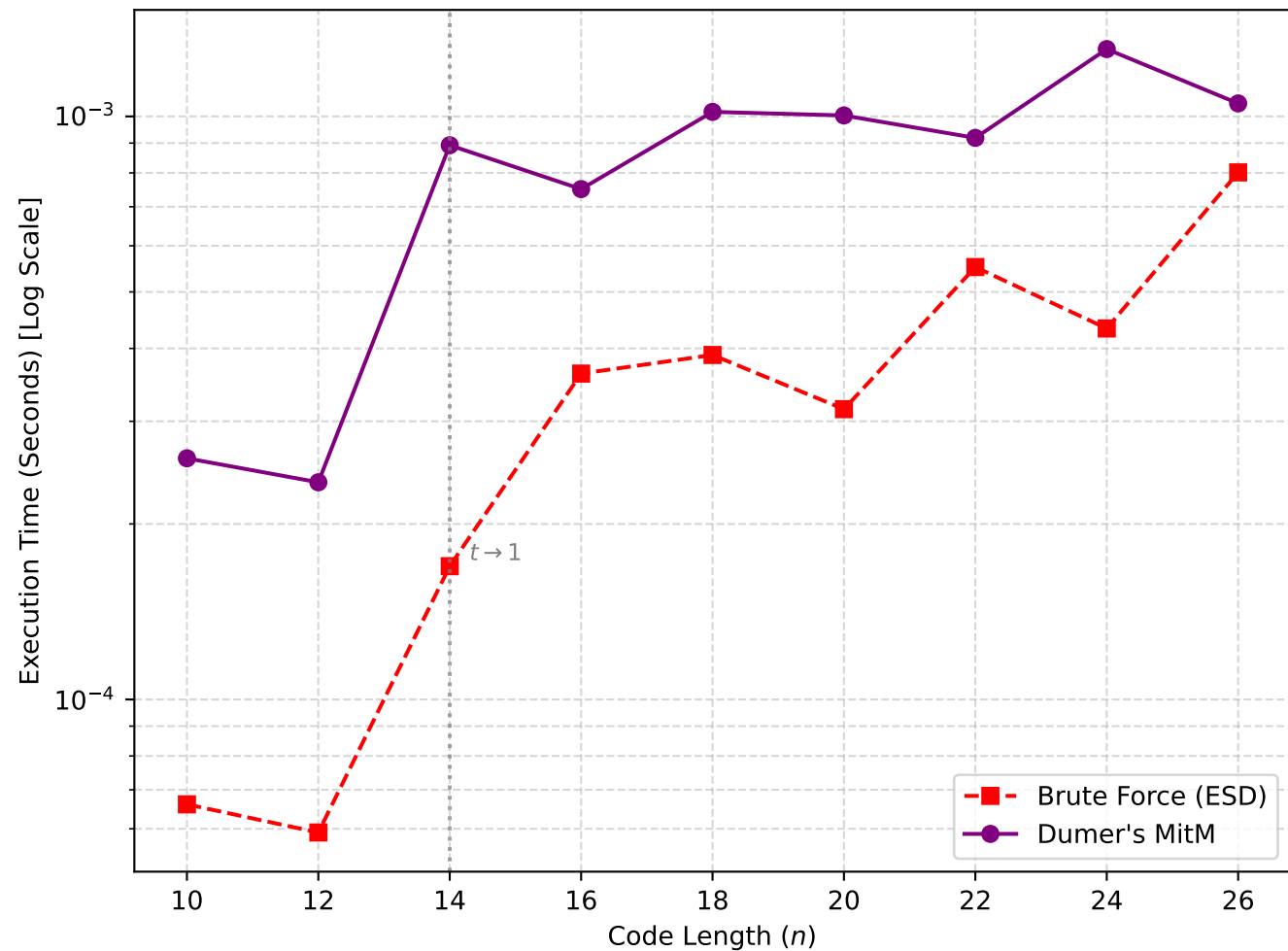
Computational Complexity: Brute Force vs Dumer's Algorithm Fixed Weight t = \lfloor (t_{GV} - 1)/2 \rfloor
