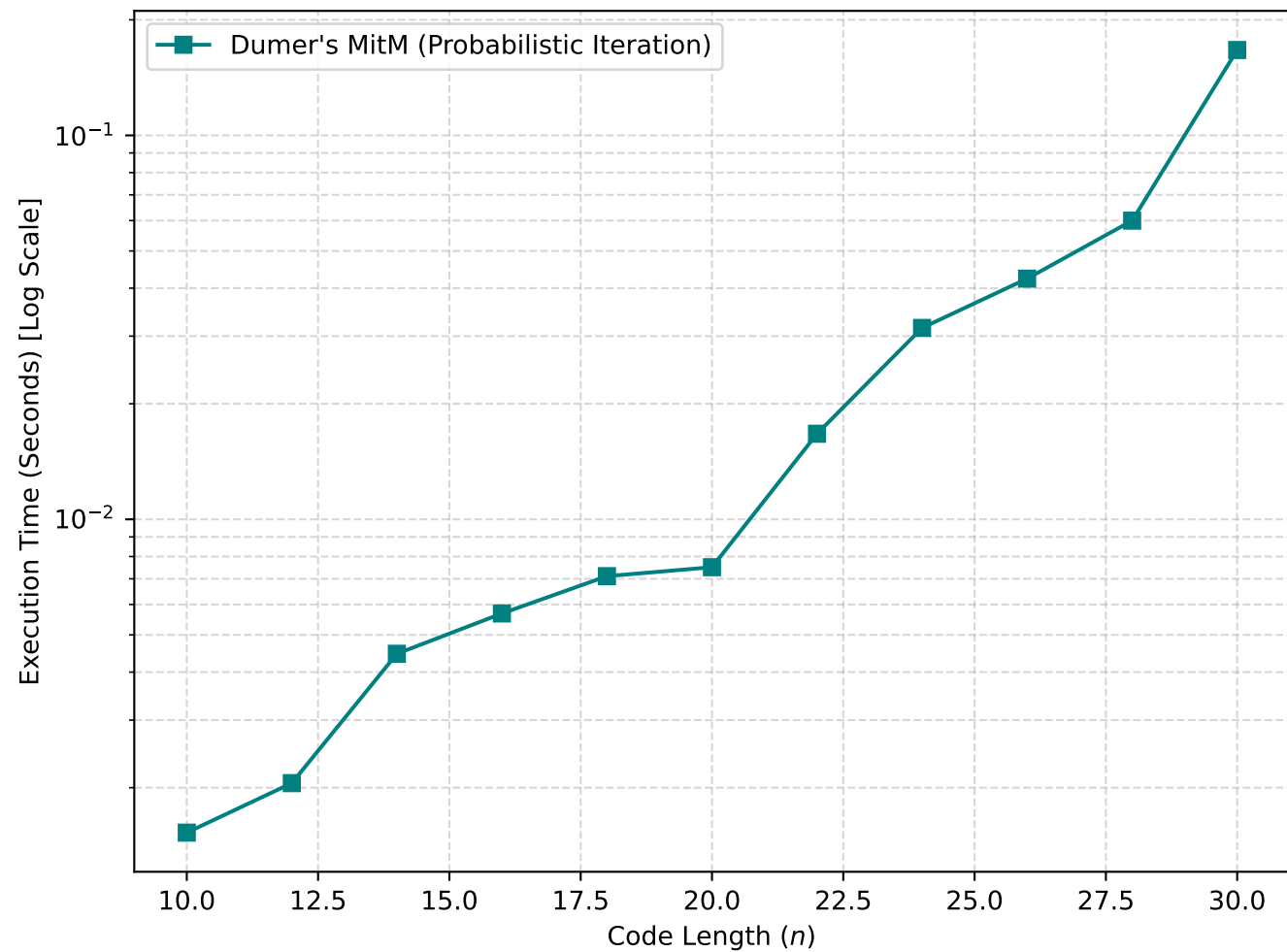
Dumer's Algorithm Benchmark: Probabilistic Search Target weight t iterating sequentially in [1, t_{GV}]
