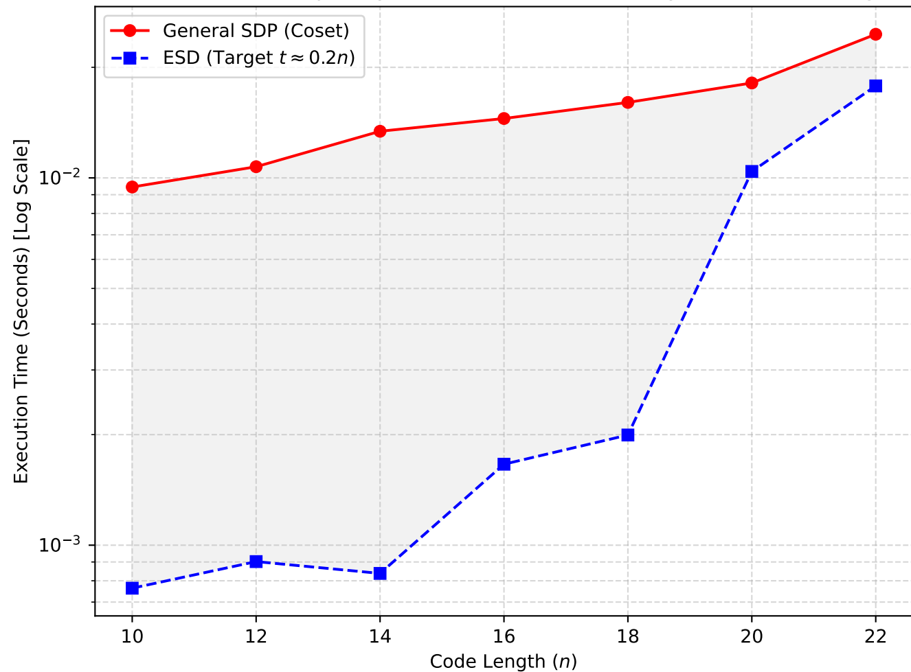
Brute-Force Complexity: General SDP vs. Exact Syndrome Decoding
