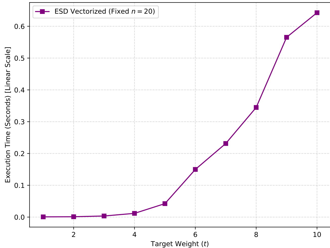
ESD Benchmark: Execution Time vs. Target Weight ( t )
