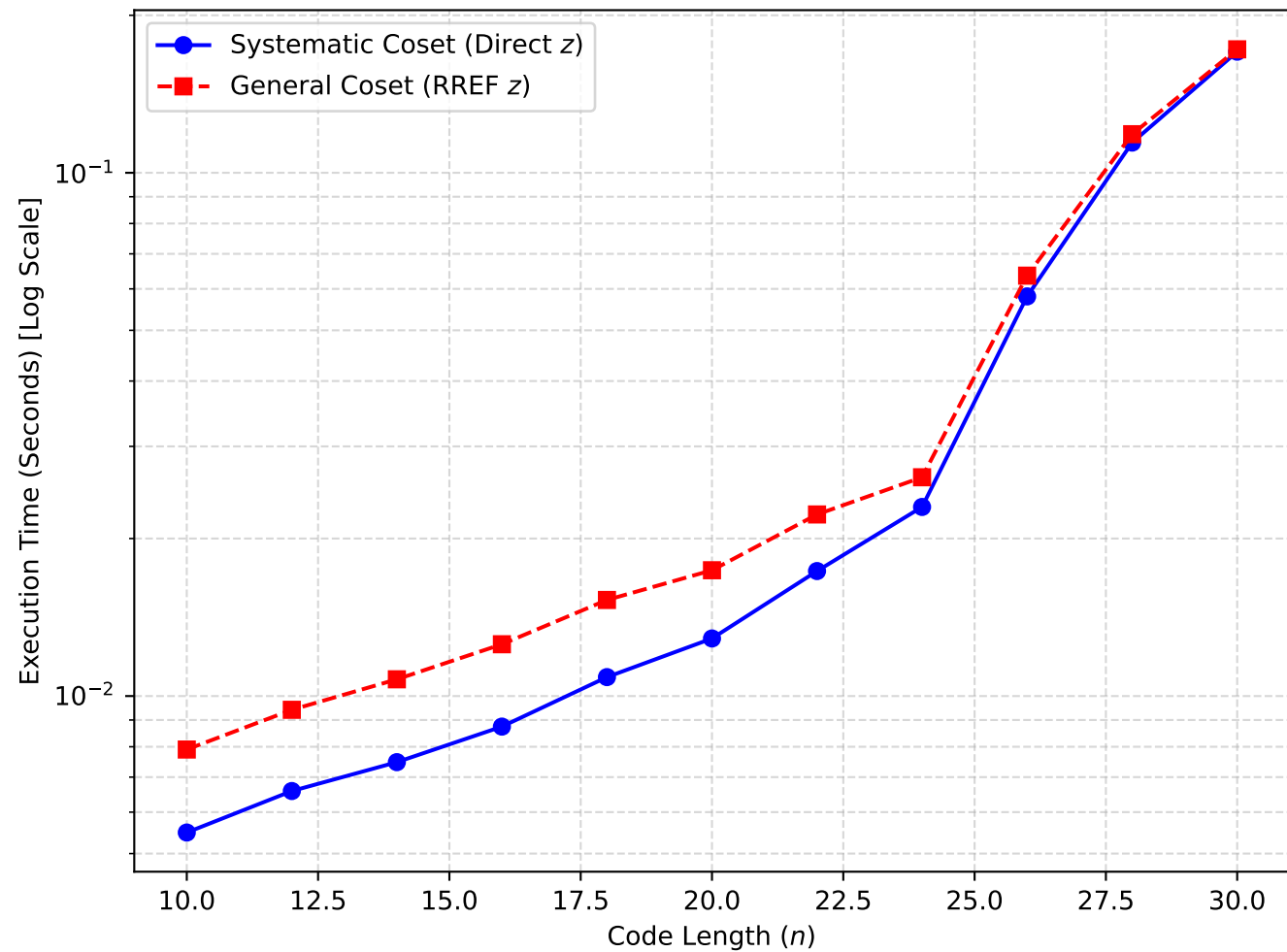
SDP Coset Benchmark: Systematic vs General Matrix Constant Rate R = 0.5
