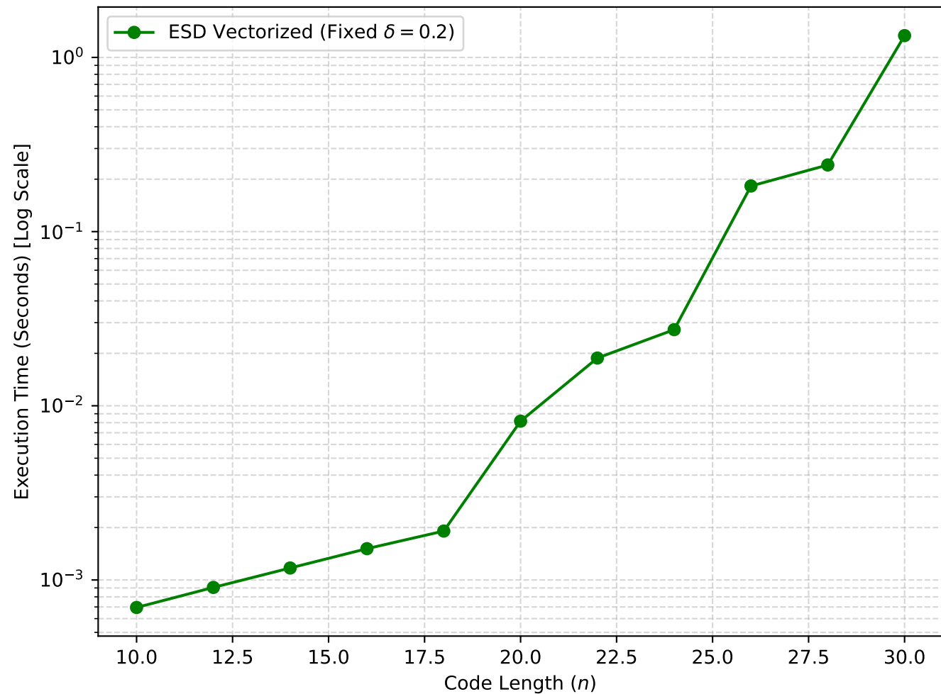
ESD Benchmark: Execution Time vs. Code Length ( n )
