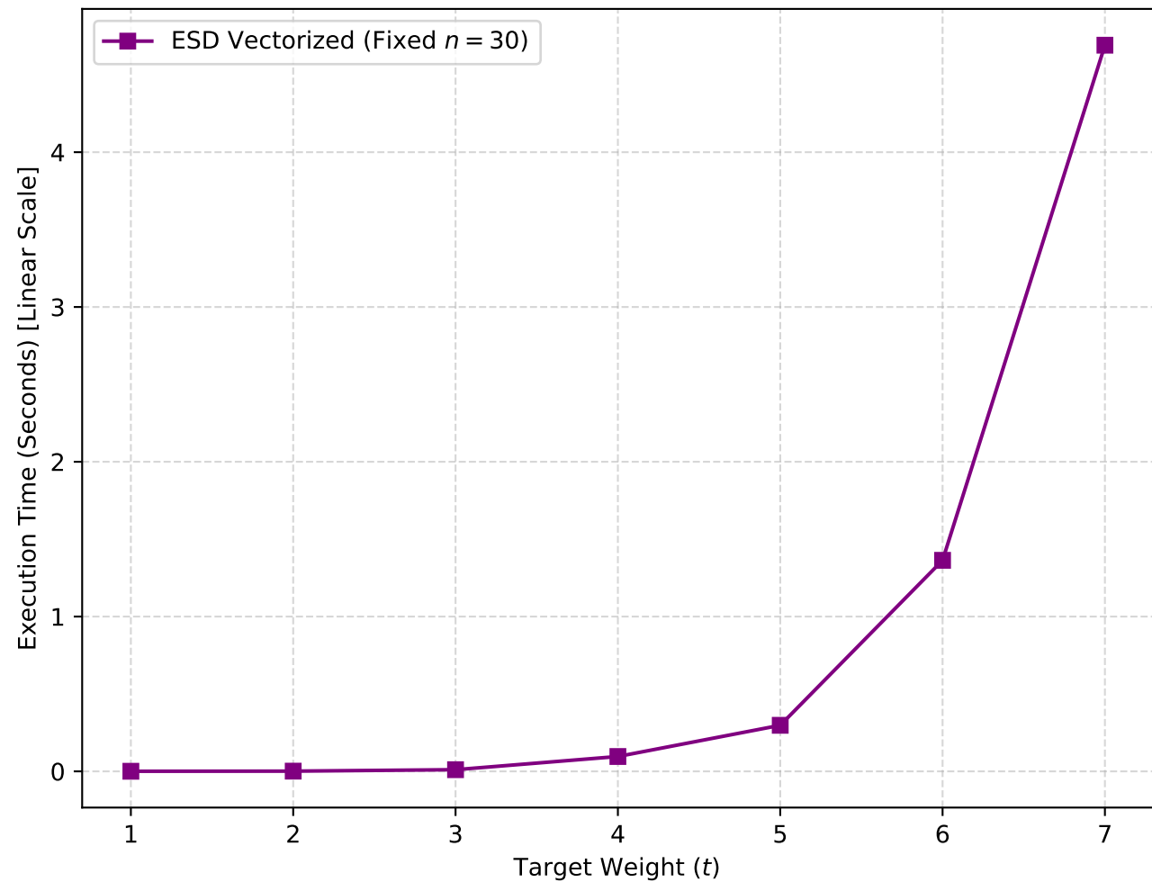
ESD Benchmark: Execution Time vs. Target Weight ( t )
