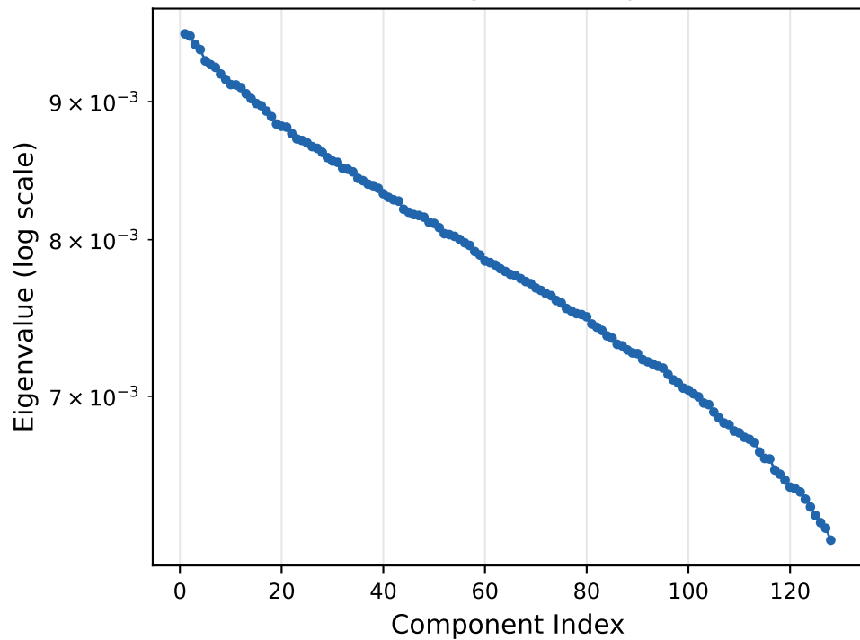
Covariance Eigenvalue Spectrum
